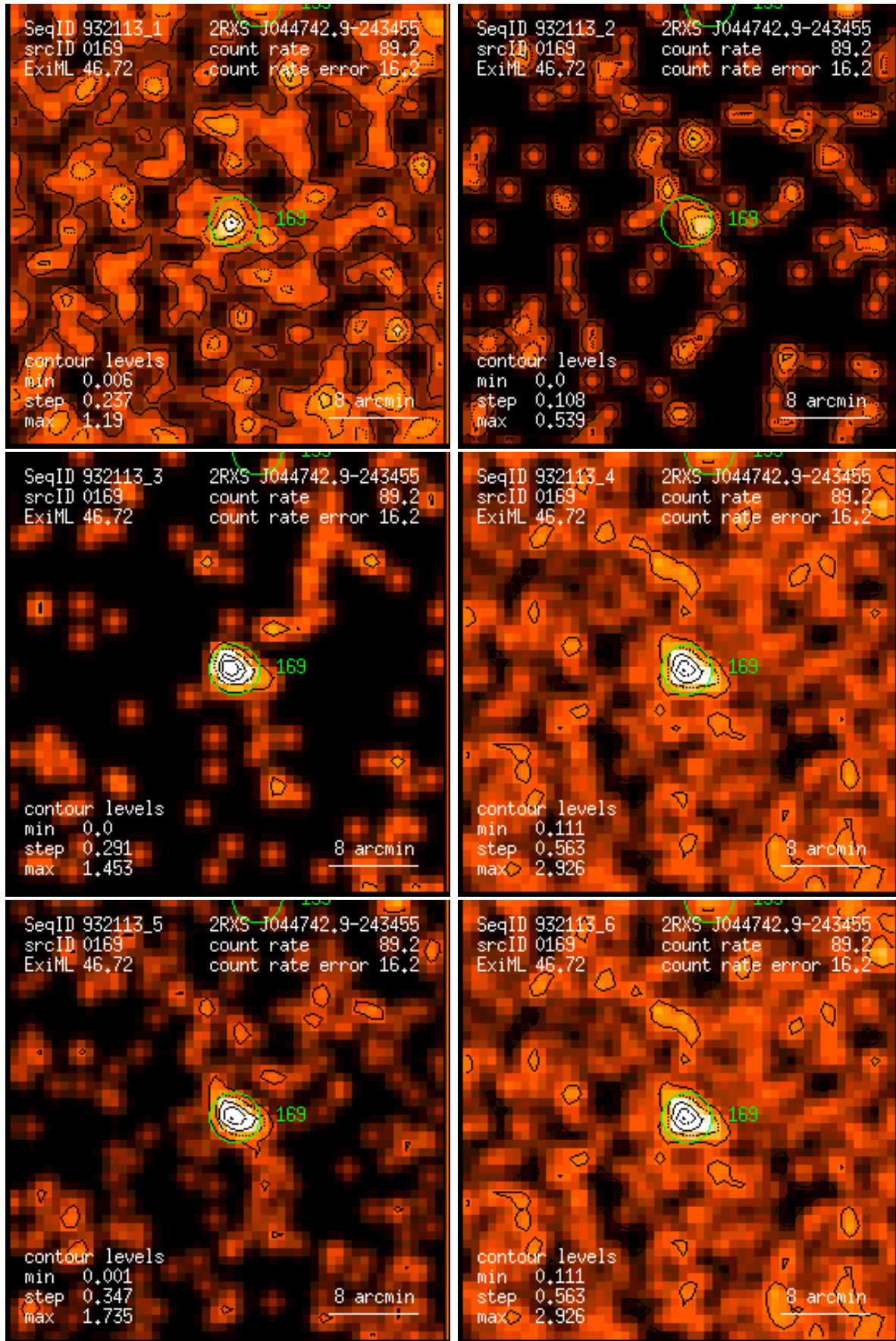
Figure 169: RASS 932113: detection 0169: band rate images, Gaussian filter: (1) PSPC channels 11 – 41, (2) 52 – 90, (3) 91 – 201, (4) 11 – 235, (5) 52 – 201, (6) 11 – 201. Broad band rates in counts/ks. Band rate contour levels in counts/ks/arcmin 2 .
