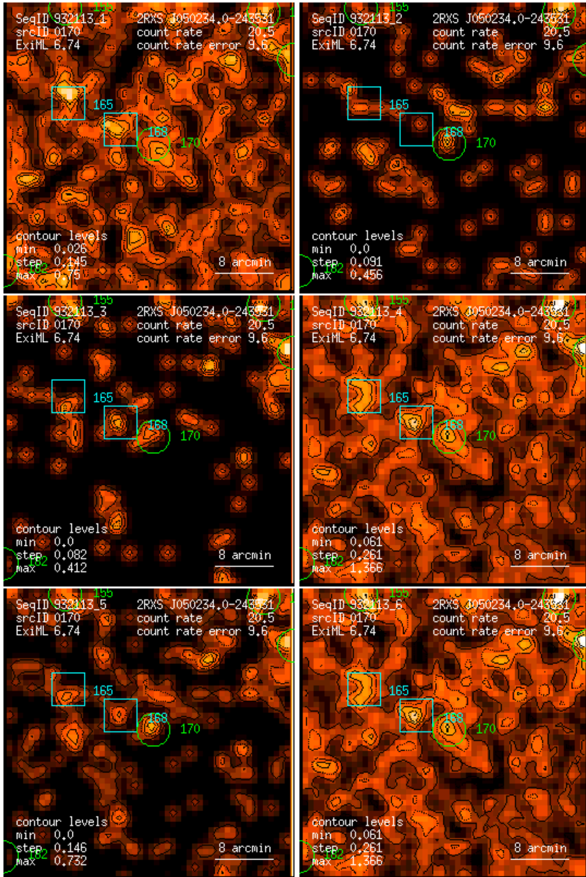
Figure 170: RASS 932113: detection 0170: band rate images, Gaussian filter: (1) PSPC channels 11 – 41, (2) 52 – 90, (3) 91 – 201, (4) 11 – 235, (5) 52 – 201, (6) 11 – 201. Broad band rates in counts/ks. Band rate contour levels in counts/ks/arcmin 2 .
