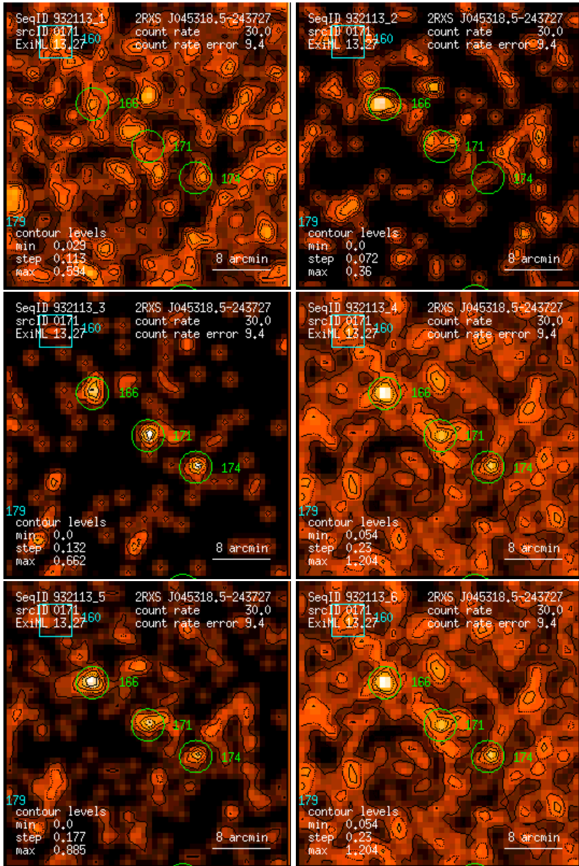
Figure 171: RASS 932113: detection 0171: band rate images, Gaussian filter: (1) PSPC channels 11 – 41, (2) 52 – 90, (3) 91 – 201, (4) 11 – 235, (5) 52 – 201, (6) 11 – 201. Broad band rates in counts/ks. Band rate contour levels in counts/ks/arcmin 2 .
