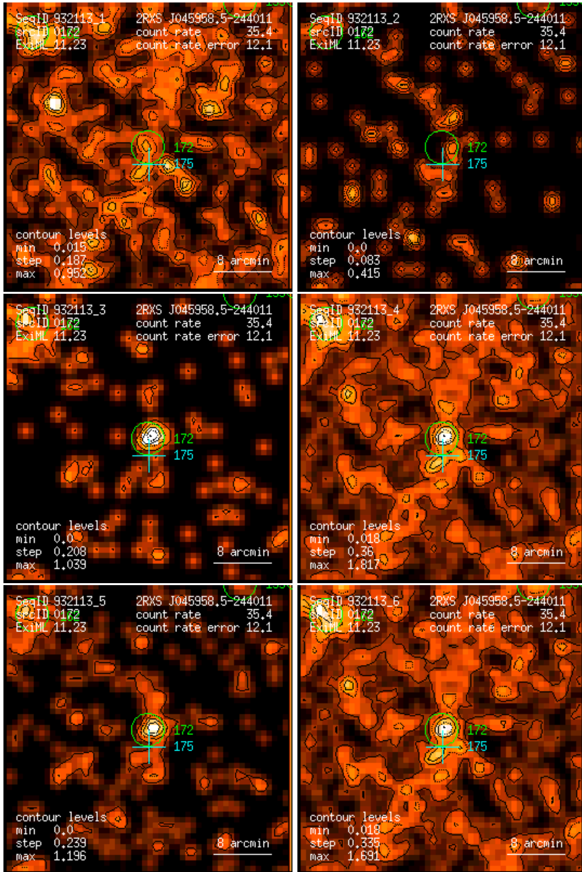
Figure 172: RASS 932113: detection 0172: band rate images, Gaussian filter: (1) PSPC channels 11 – 41, (2) 52 – 90, (3) 91 – 201, (4) 11 – 235, (5) 52 – 201, (6) 11 – 201. Broad band rates in counts/ks. Band rate contour levels in counts/ks/arcmin 2 .
