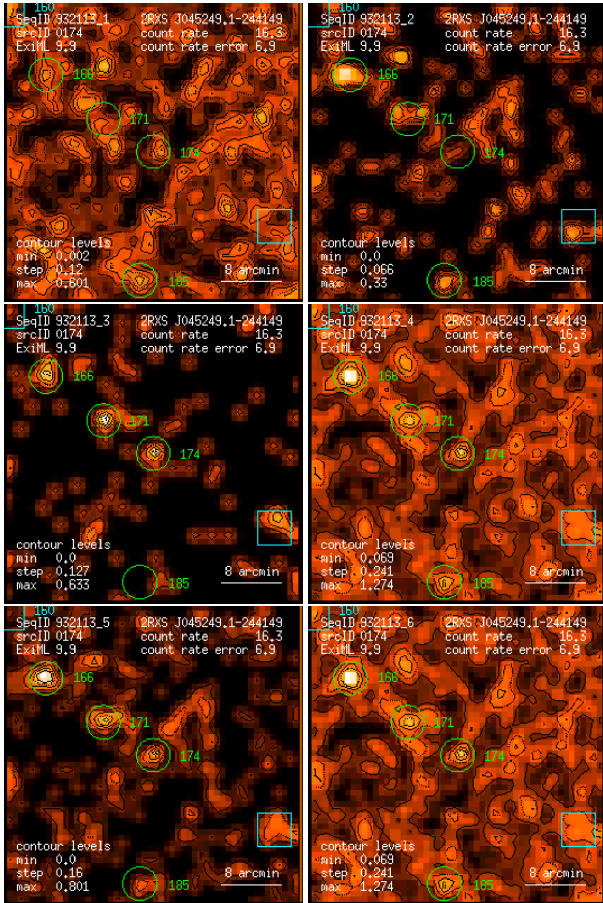
Figure 174: RASS 932113: detection 0174: band rate images, Gaussian filter: (1) PSPC channels 11 – 41, (2) 52 – 90, (3) 91 – 201, (4) 11 – 235, (5) 52 – 201, (6) 11 – 201. Broad band rates in counts/ks. Band rate contour levels in counts/ks/arcmin 2 .
