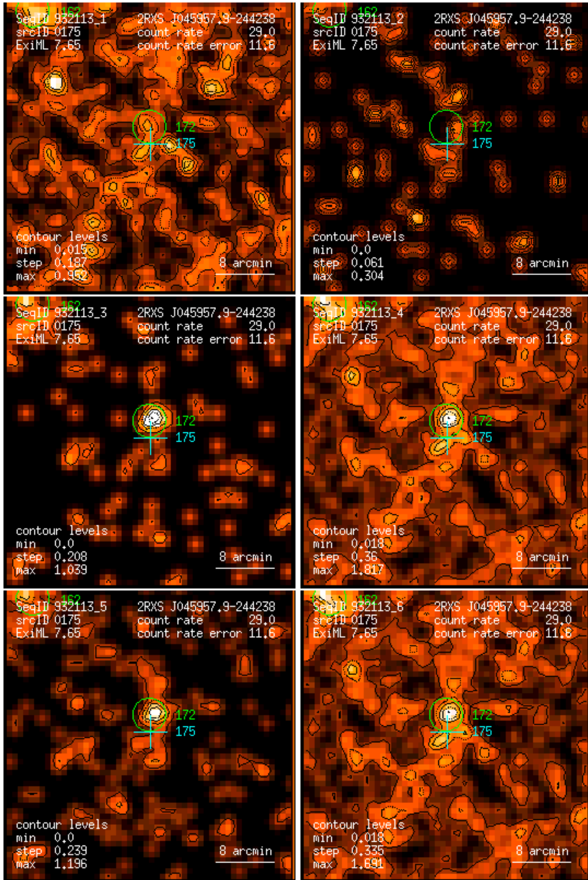
Figure 175: RASS 932113: detection 0175: band rate images, Gaussian filter: (1) PSPC channels 11 – 41, (2) 52 – 90, (3) 91 – 201, (4) 11 – 235, (5) 52 – 201, (6) 11 – 201. Broad band rates in counts/ks. Band rate contour levels in counts/ks/arcmin 2 .
