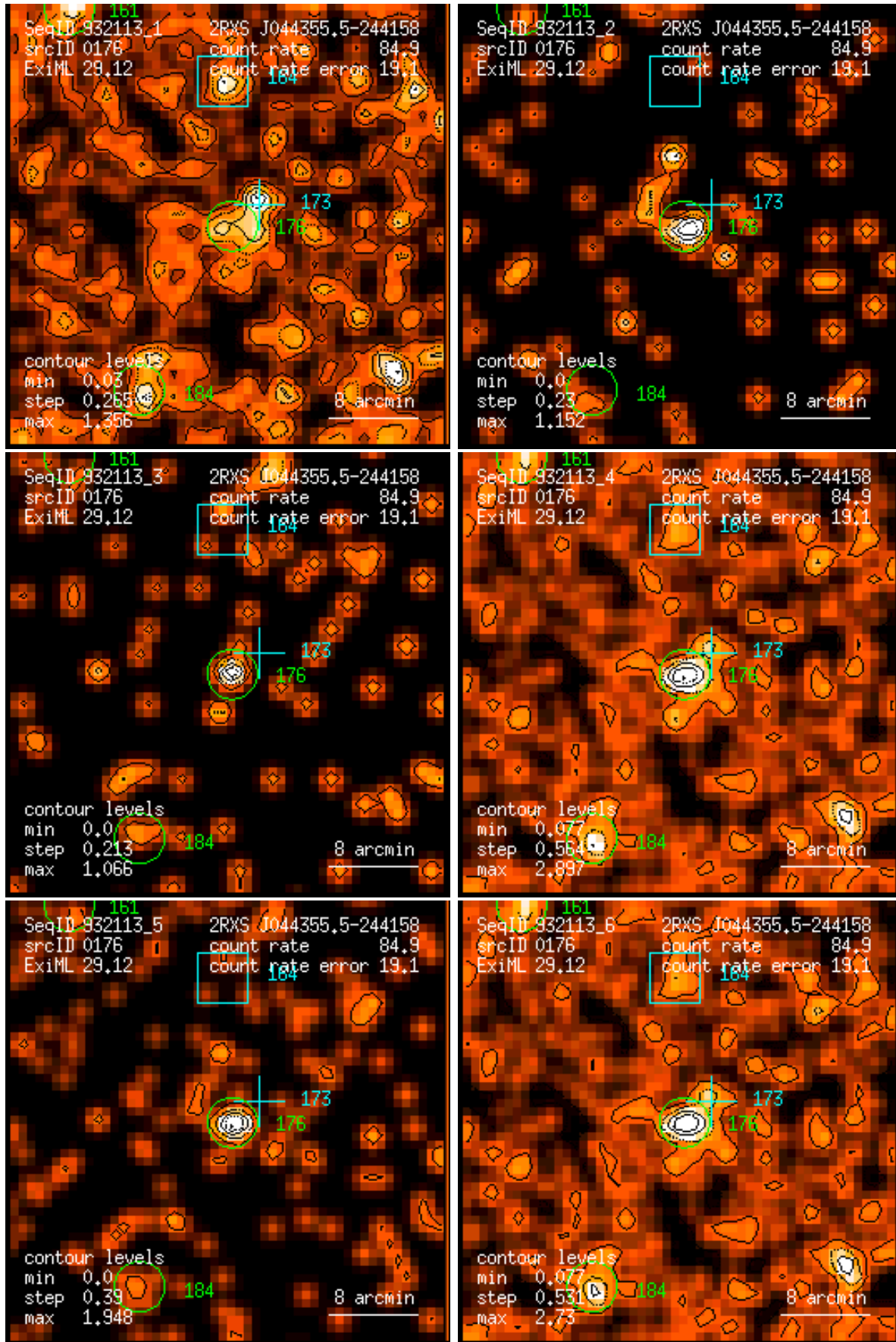
Figure 176: RASS 932113: detection 0176: band rate images, Gaussian filter: (1) PSPC channels 11 – 41, (2) 52 – 90, (3) 91 – 201, (4) 11 – 235, (5) 52 – 201, (6) 11 – 201. Broad band rates in counts/ks. Band rate contour levels in counts/ks/arcmin 2 .
