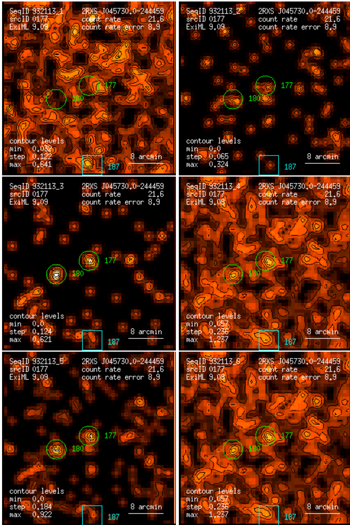
Figure 177: RASS 932113: detection 0177: band rate images, Gaussian filter: (1) PSPC channels 11 – 41, (2) 52 – 90, (3) 91 – 201, (4) 11 – 235, (5) 52 – 201, (6) 11 – 201. Broad band rates in counts/ks. Band rate contour levels in counts/ks/arcmin 2 .
