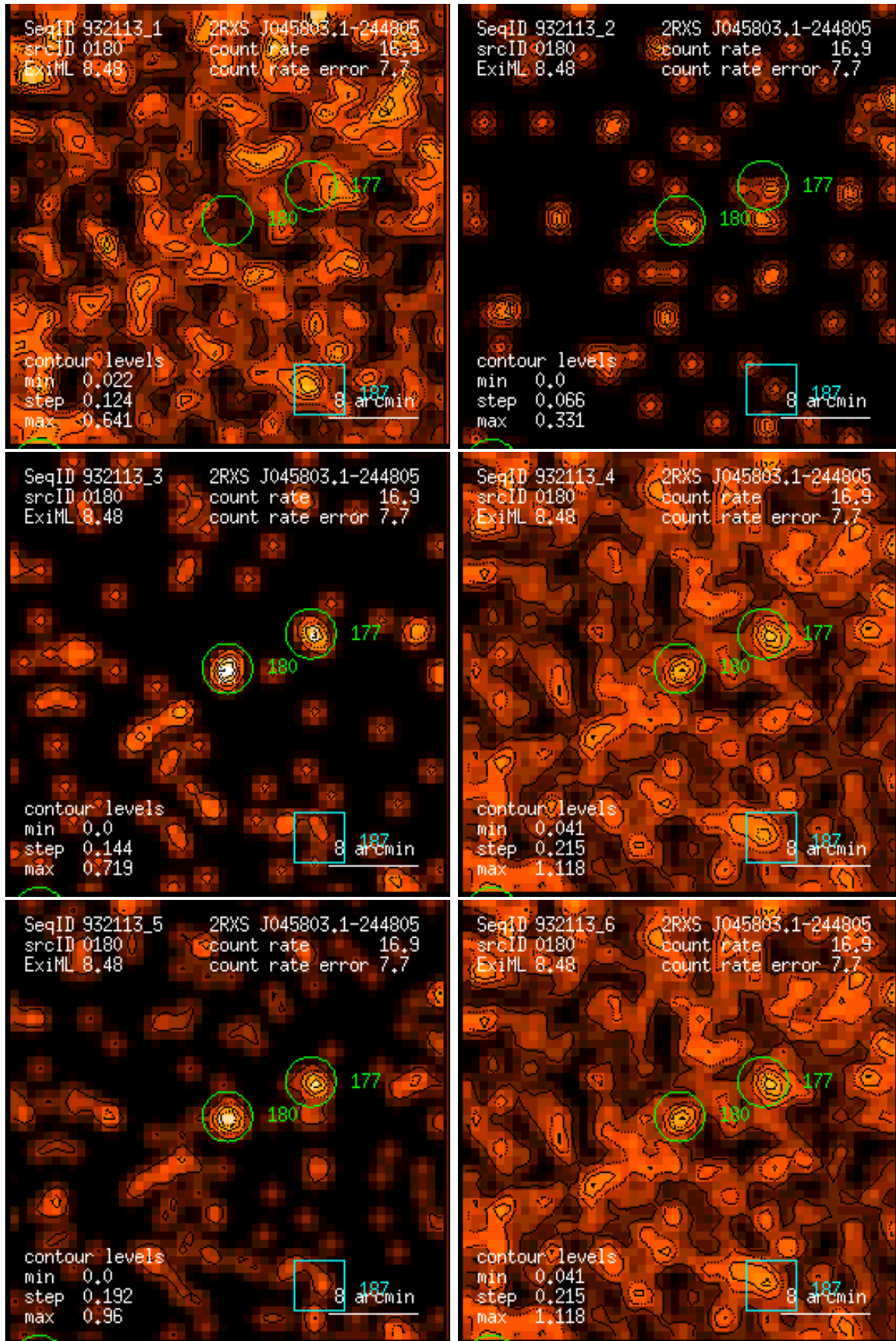
Figure 180: RASS 932113: detection 0180: band rate images, Gaussian filter: (1) PSPC channels 11 – 41, (2) 52 – 90, (3) 91 – 201, (4) 11 – 235, (5) 52 – 201, (6) 11 – 201. Broad band rates in counts/ks. Band rate contour levels in counts/ks/arcmin 2 .
