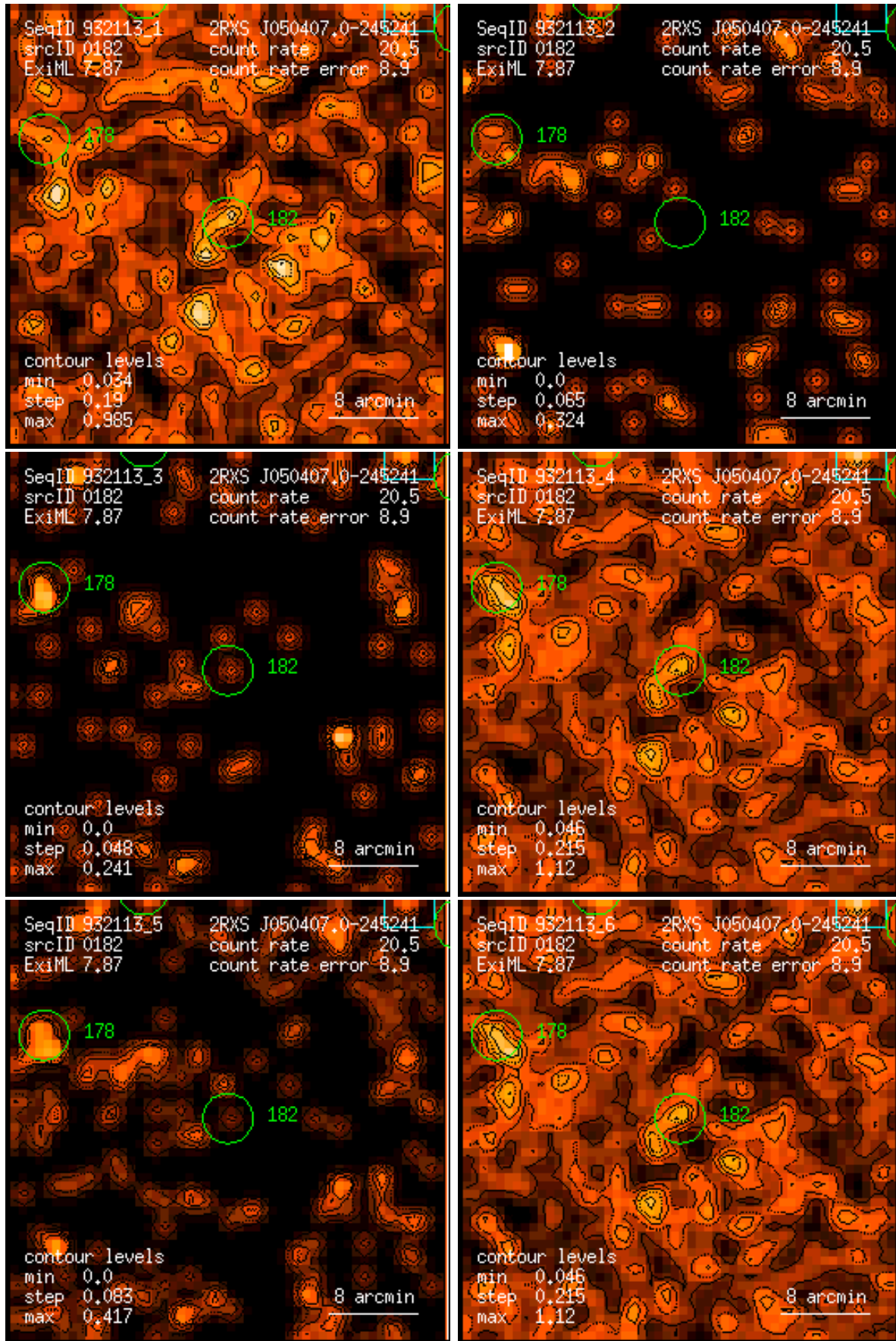
Figure 182: RASS 932113: detection 0182: band rate images, Gaussian filter: (1) PSPC channels 11 – 41, (2) 52 – 90, (3) 91 – 201, (4) 11 – 235, (5) 52 – 201, (6) 11 – 201. Broad band rates in counts/ks. Band rate contour levels in counts/ks/arcmin 2 .
