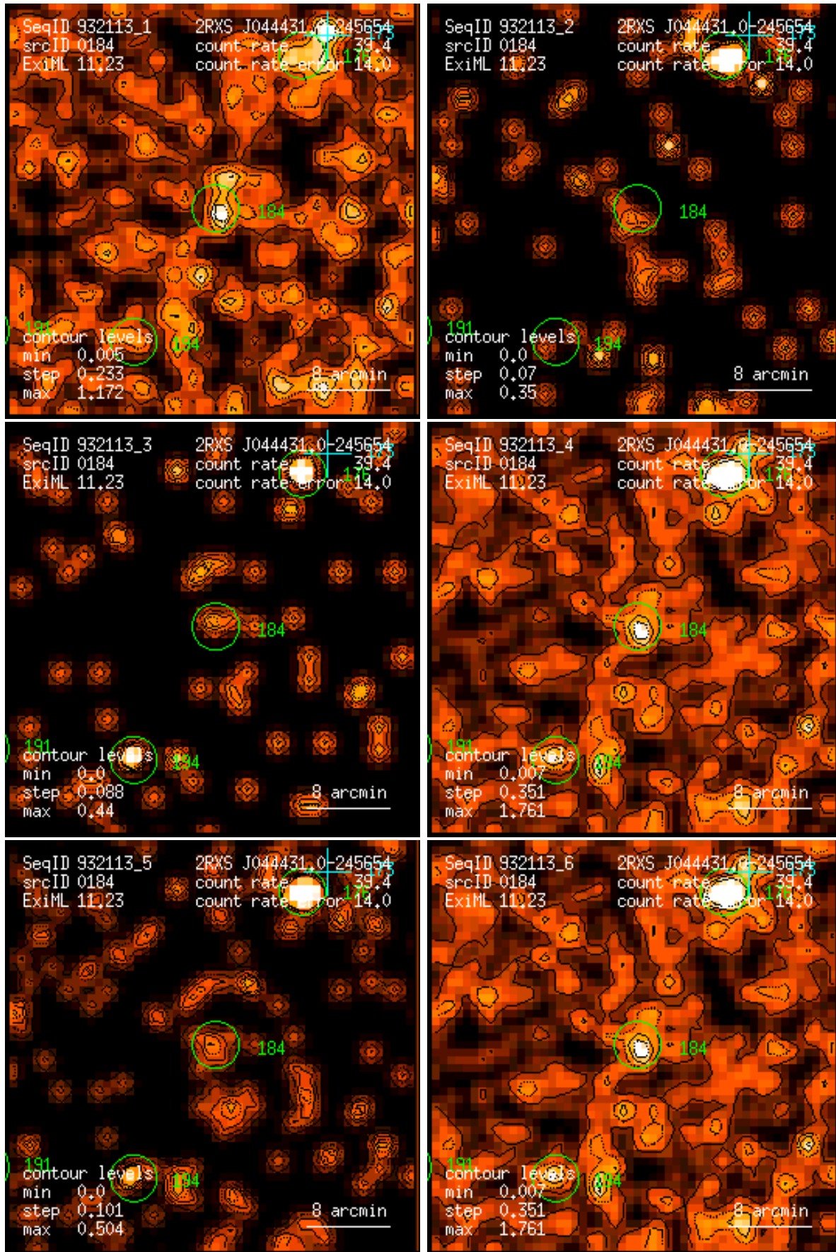
Figure 184: RASS 932113: detection 0184: band rate images, Gaussian filter: (1) PSPC channels 11 – 41, (2) 52 – 90, (3) 91 – 201, (4) 11 – 235, (5) 52 – 201, (6) 11 – 201. Broad band rates in counts/ks. Band rate contour levels in counts/ks/arcmin 2 .
