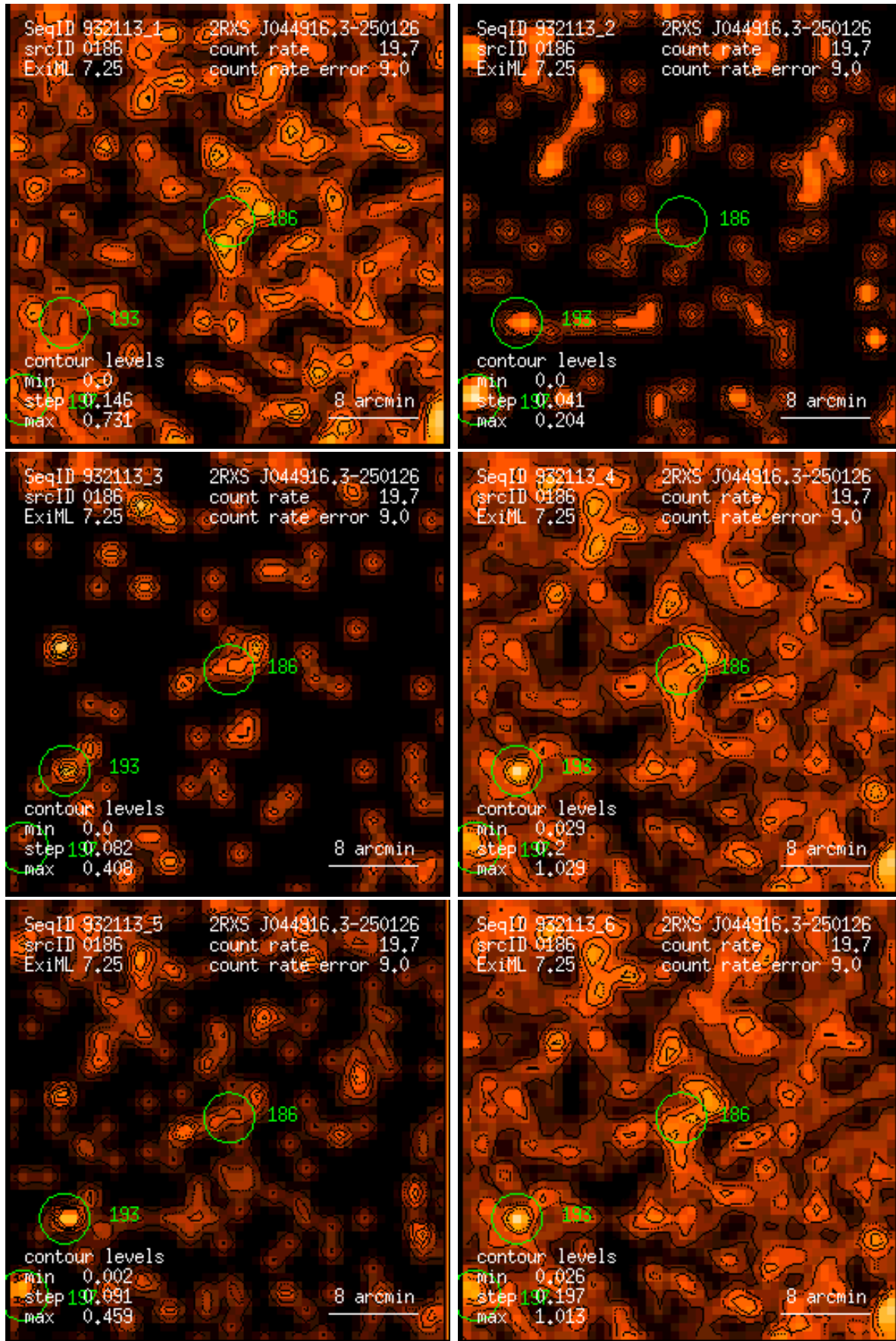
Figure 186: RASS 932113: detection 0186: band rate images, Gaussian filter: (1) PSPC channels 11 – 41, (2) 52 – 90, (3) 91 – 201, (4) 11 – 235, (5) 52 – 201, (6) 11 – 201. Broad band rates in counts/ks. Band rate contour levels in counts/ks/arcmin 2 .
