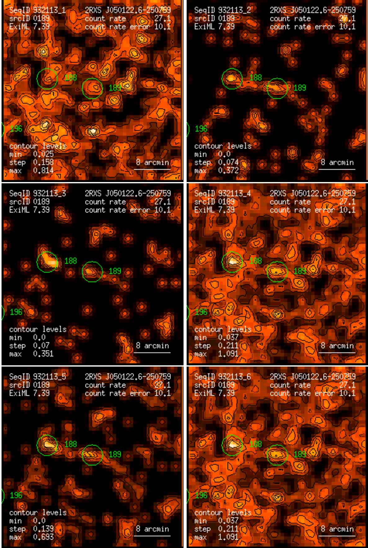
Figure 189: RASS 932113: detection 0189: band rate images, Gaussian filter: (1) PSPC channels 11 – 41, (2) 52 – 90, (3) 91 – 201, (4) 11 – 235, (5) 52 – 201, (6) 11 – 201. Broad band rates in counts/ks. Band rate contour levels in counts/ks/arcmin 2 .
