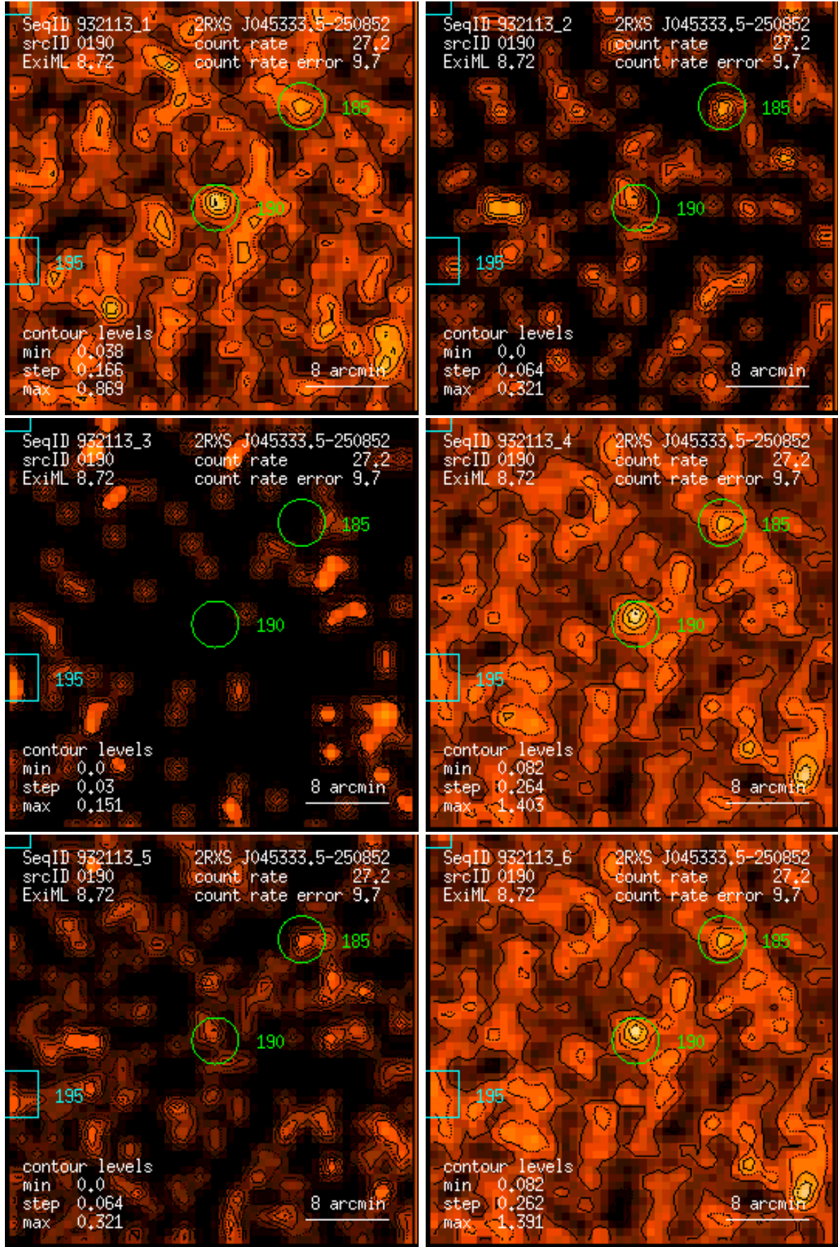
Figure 190: RASS 932113: detection 0190: band rate images, Gaussian filter: (1) PSPC channels 11 – 41, (2) 52 – 90, (3) 91 – 201, (4) 11 – 235, (5) 52 – 201, (6) 11 – 201. Broad band rates in counts/ks. Band rate contour levels in counts/ks/arcmin 2 .
