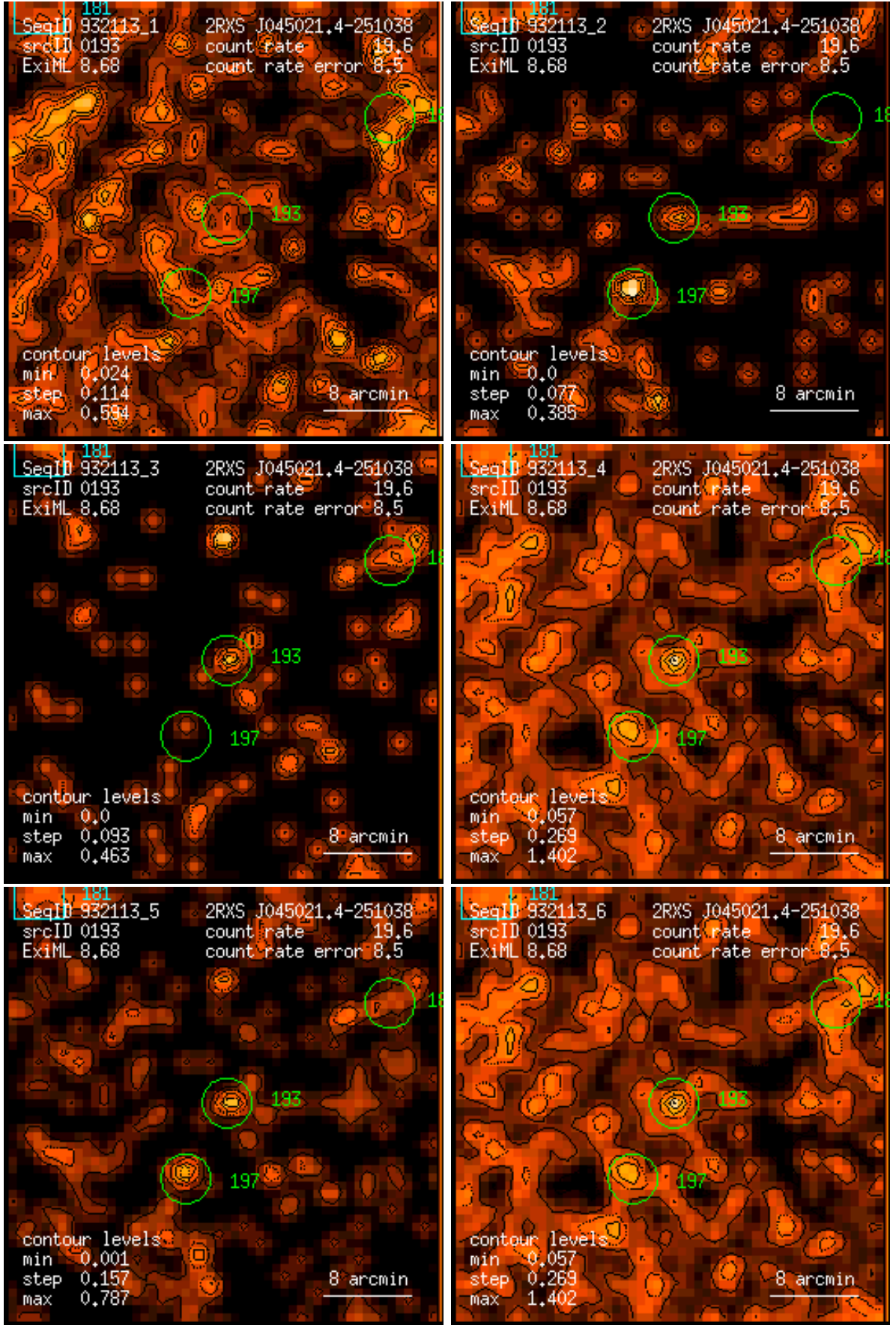
Figure 193: RASS 932113: detection 0193: band rate images, Gaussian filter: (1) PSPC channels 11 – 41, (2) 52 – 90, (3) 91 – 201, (4) 11 – 235, (5) 52 – 201, (6) 11 – 201. Broad band rates in counts/ks. Band rate contour levels in counts/ks/arcmin 2 .
