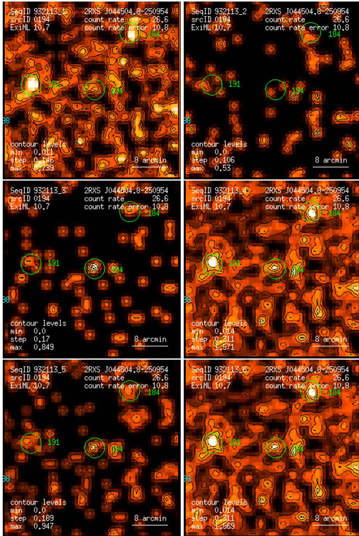
Figure 194: RASS 932113: detection 0194: band rate images, Gaussian filter: (1) PSPC channels 11 – 41, (2) 52 – 90, (3) 91 – 201, (4) 11 – 235, (5) 52 – 201, (6) 11 – 201. Broad band rates in counts/ks. Band rate contour levels in counts/ks/arcmin 2 .
