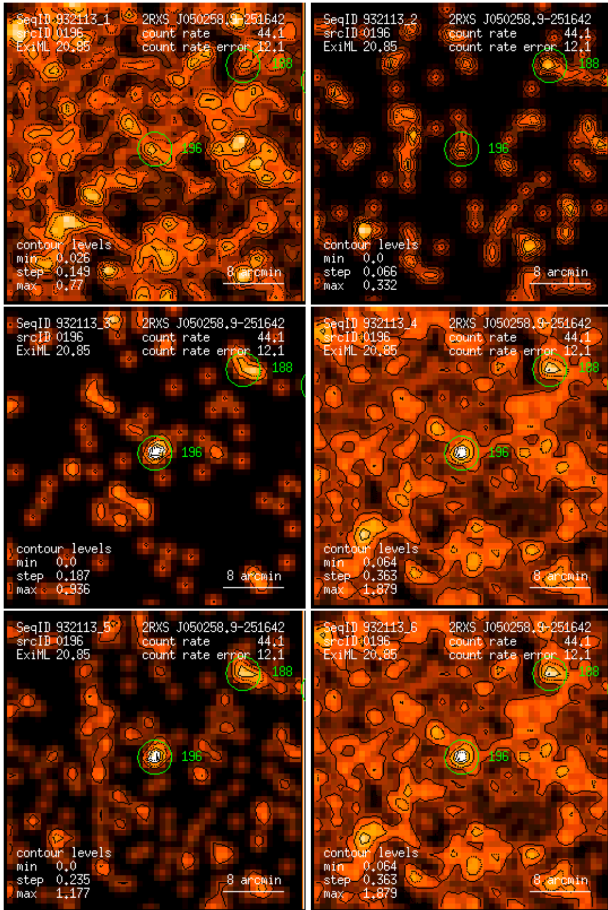
Figure 196: RASS 932113: detection 0196: band rate images, Gaussian filter: (1) PSPC channels 11 – 41, (2) 52 – 90, (3) 91 – 201, (4) 11 – 235, (5) 52 – 201, (6) 11 – 201. Broad band rates in counts/ks. Band rate contour levels in counts/ks/arcmin 2 .
