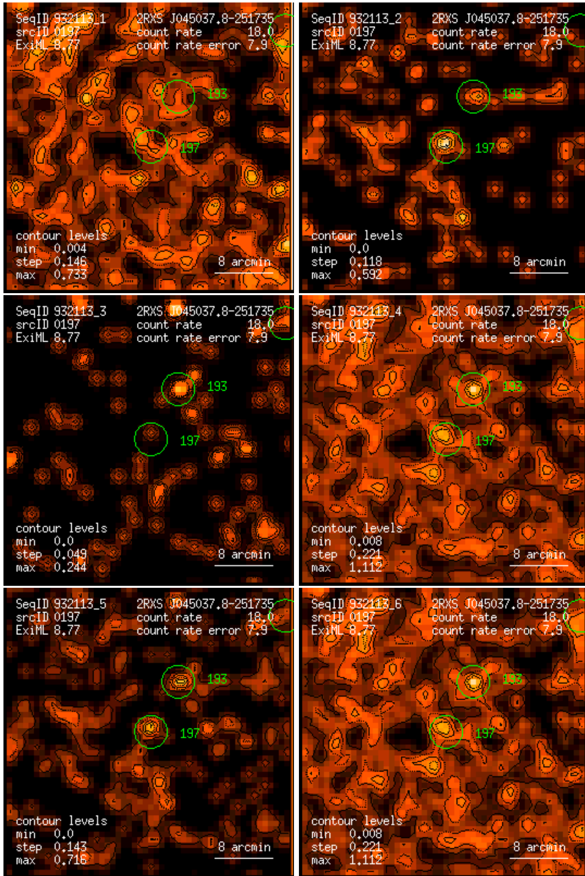
Figure 197: RASS 932113: detection 0197: band rate images, Gaussian filter: (1) PSPC channels 11 – 41, (2) 52 – 90, (3) 91 – 201, (4) 11 – 235, (5) 52 – 201, (6) 11 – 201. Broad band rates in counts/ks. Band rate contour levels in counts/ks/arcmin 2 .
