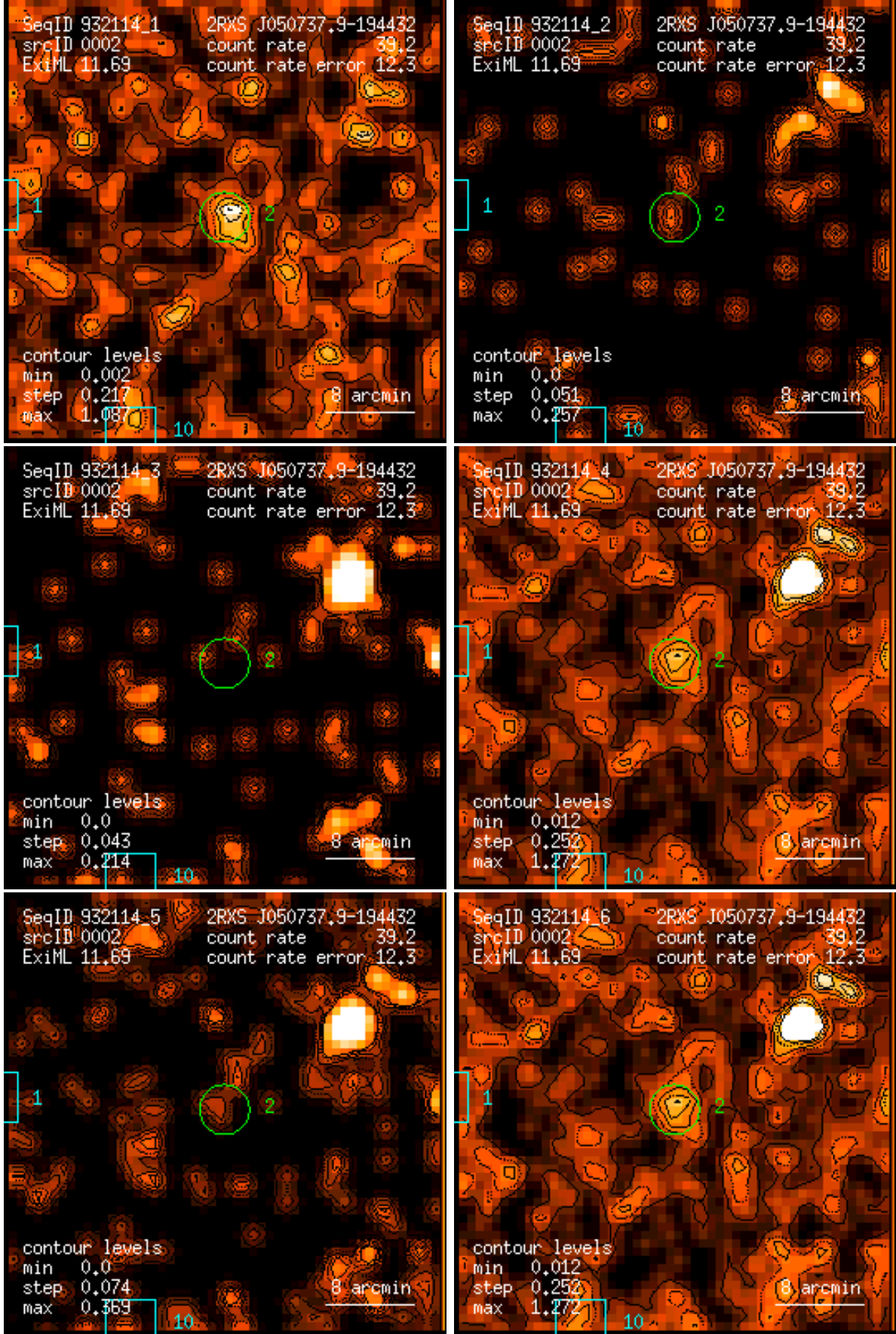
Figure 2: RASS 932114: detection 0002: band rate images, Gaussian filter: (1) PSPC channels 11 – 41, (2) 52 – 90, (3) 91 – 201, (4) 11 – 235, (5) 52 – 201, (6) 11 – 201. Broad band rates in counts/ks. Band rate contour levels in counts/ks/arcmin 2 .
