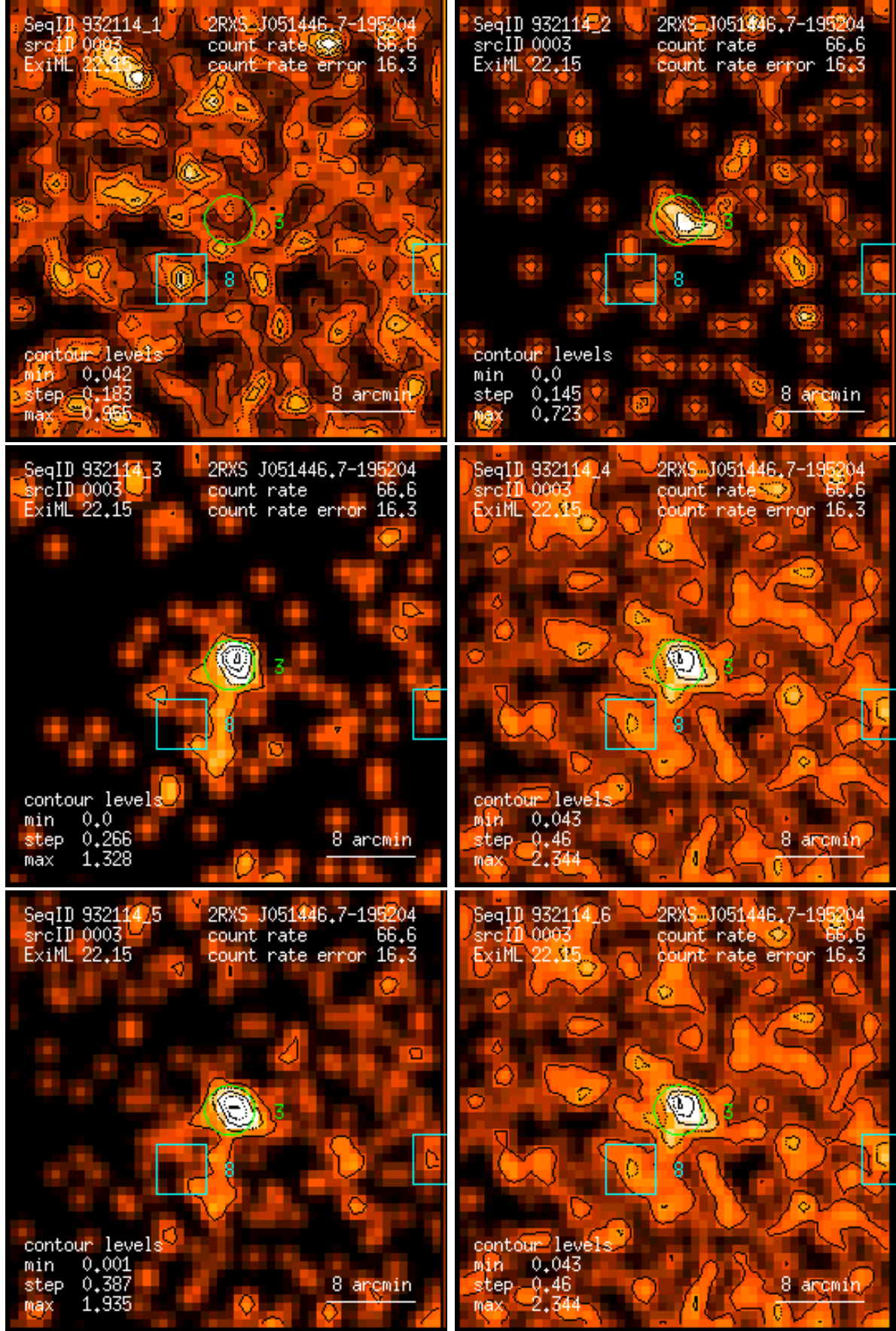
Figure 3: RASS 932114: detection 0003: band rate images, Gaussian filter: (1) PSPC channels 11 – 41, (2) 52 – 90, (3) 91 – 201, (4) 11 – 235, (5) 52 – 201, (6) 11 – 201. Broad band rates in counts/ks. Band rate contour levels in counts/ks/arcmin 2 .
