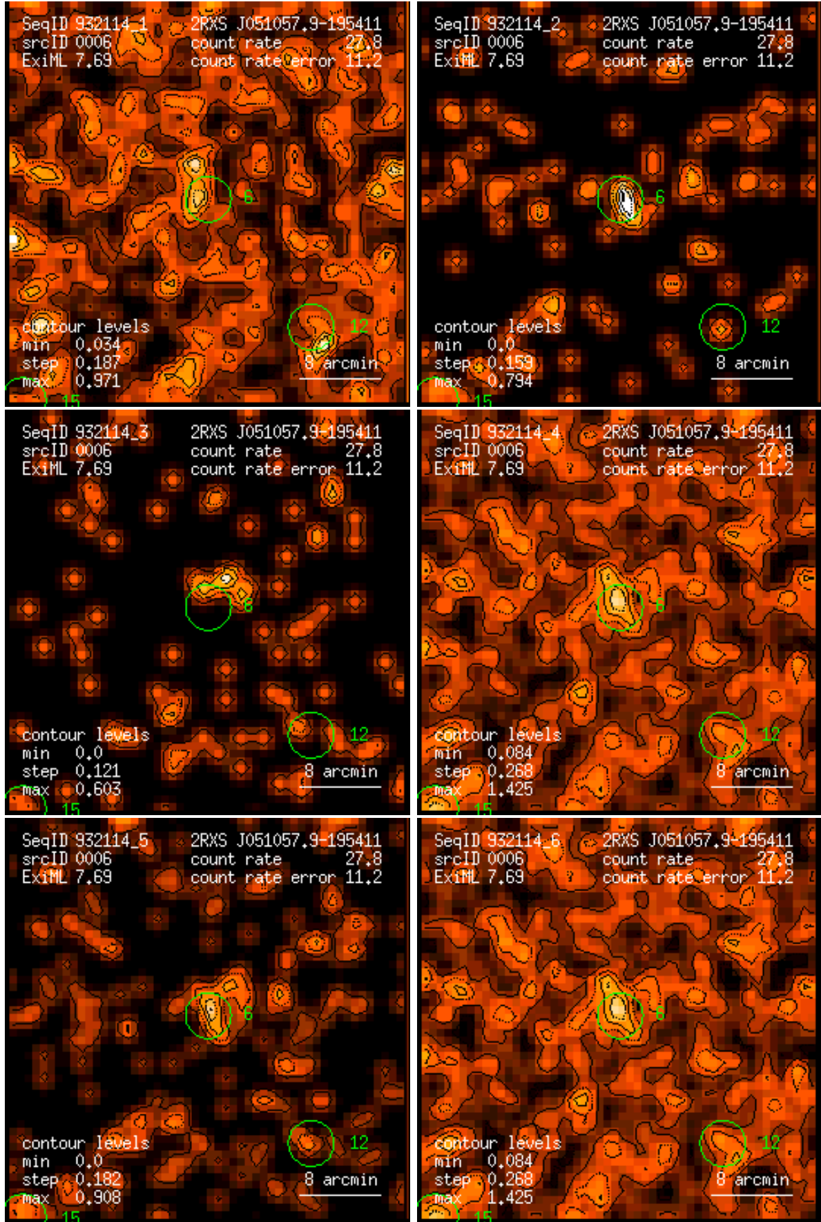
Figure 6: RASS 932114: detection 0006: band rate images, Gaussian filter: (1) PSPC channels 11 – 41, (2) 52 – 90, (3) 91 – 201, (4) 11 – 235, (5) 52 – 201, (6) 11 – 201. Broad band rates in counts/ks. Band rate contour levels in counts/ks/arcmin 2 .
