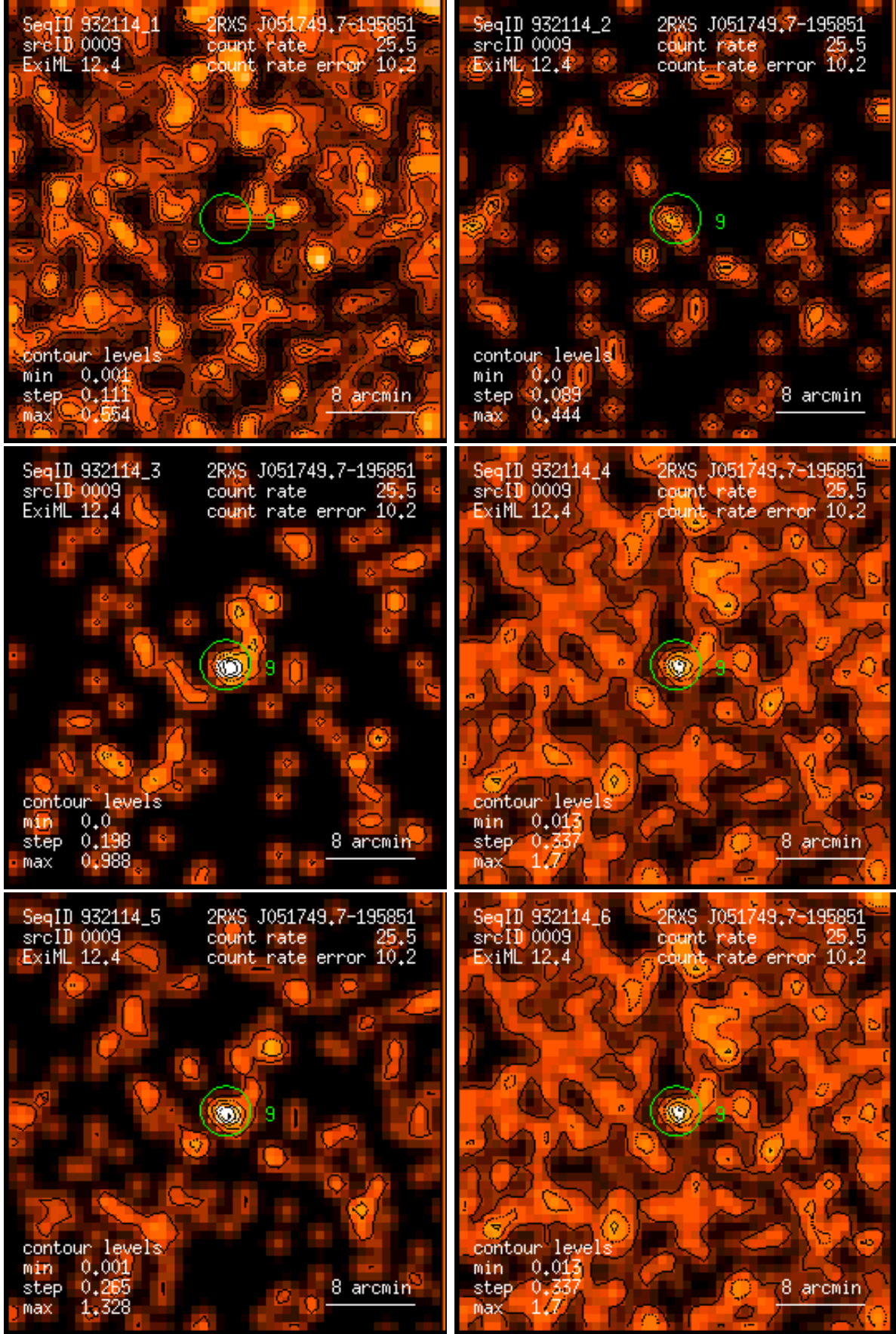
Figure 9: RASS 932114: detection 0009: band rate images, Gaussian filter: (1) PSPC channels 11 – 41, (2) 52 – 90, (3) 91 – 201, (4) 11 – 235, (5) 52 – 201, (6) 11 – 201. Broad band rates in counts/ks. Band rate contour levels in counts/ks/arcmin 2 .
