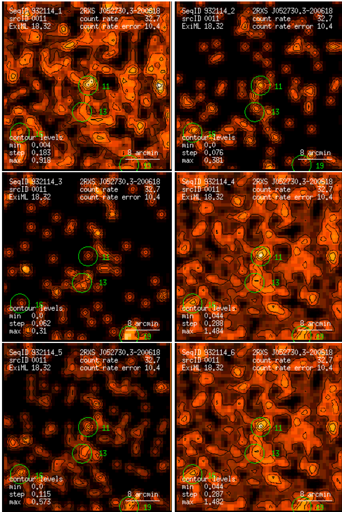
Figure 11: RASS 932114: detection 0011: band rate images, Gaussian filter: (1) PSPC channels 11 – 41, (2) 52 – 90, (3) 91 – 201, (4) 11 – 235, (5) 52 – 201, (6) 11 – 201. Broad band rates in counts/ks. Band rate contour levels in counts/ks/arcmin 2 .
