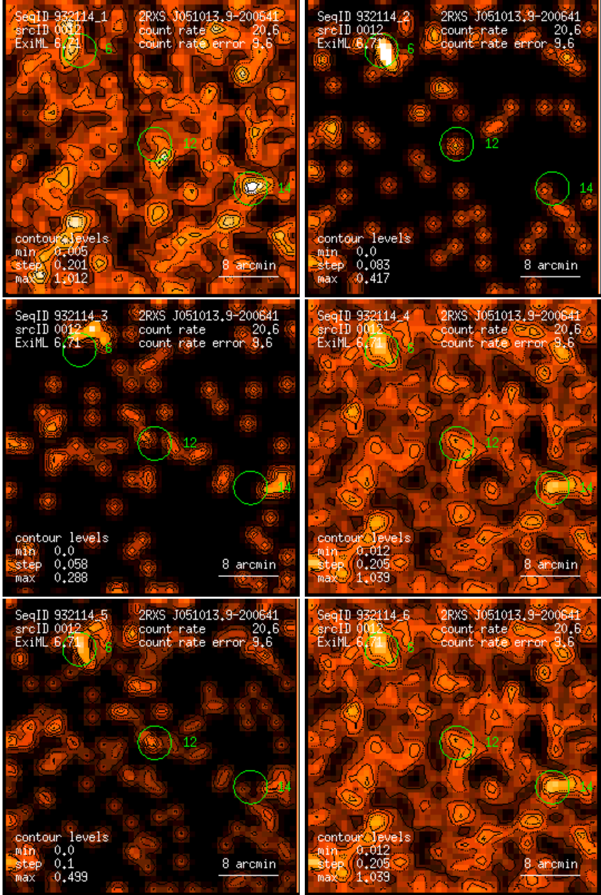
Figure 12: RASS 932114: detection 0012: band rate images, Gaussian filter: (1) PSPC channels 11 – 41, (2) 52 – 90, (3) 91 – 201, (4) 11 – 235, (5) 52 – 201, (6) 11 – 201. Broad band rates in counts/ks. Band rate contour levels in counts/ks/arcmin 2 .
