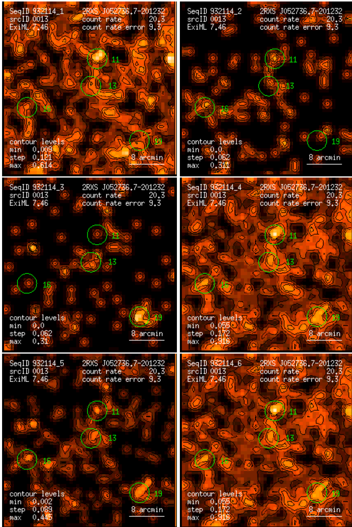
Figure 13: RASS 932114: detection 0013: band rate images, Gaussian filter: (1) PSPC channels 11 – 41, (2) 52 – 90, (3) 91 – 201, (4) 11 – 235, (5) 52 – 201, (6) 11 – 201. Broad band rates in counts/ks. Band rate contour levels in counts/ks/arcmin 2 .
