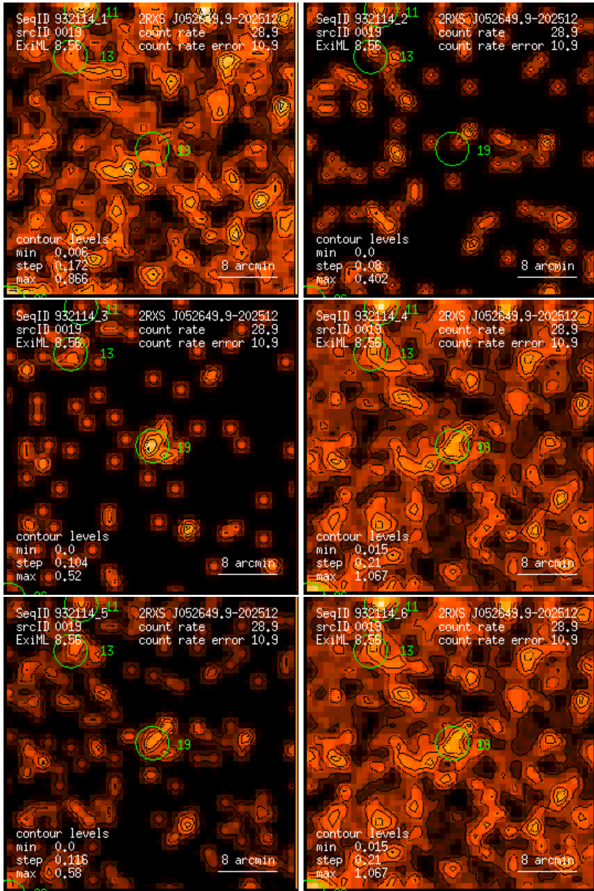
Figure 19: RASS 932114: detection 0019: band rate images, Gaussian filter: (1) PSPC channels 11 – 41, (2) 52 – 90, (3) 91 – 201, (4) 11 – 235, (5) 52 – 201, (6) 11 – 201. Broad band rates in counts/ks. Band rate contour levels in counts/ks/arcmin 2 .
