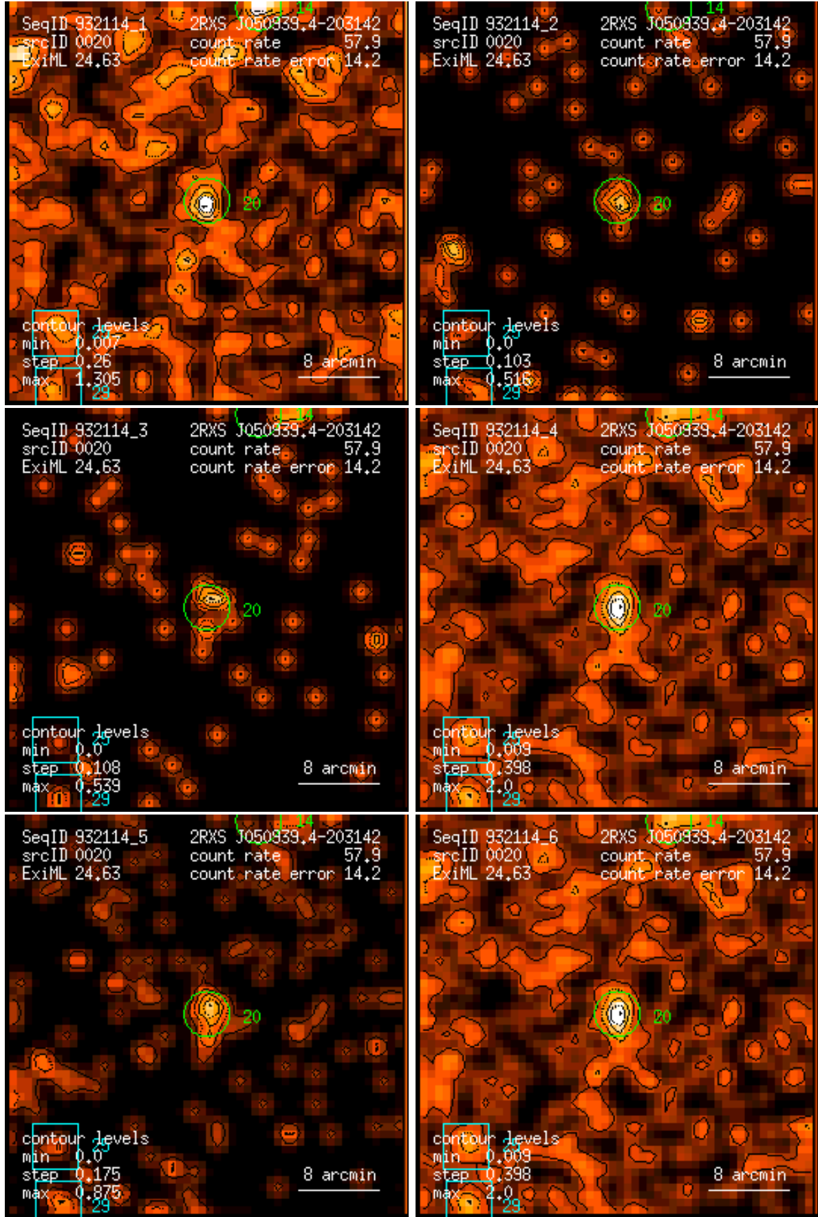
Figure 20: RASS 932114: detection 0020: band rate images, Gaussian filter: (1) PSPC channels 11 – 41, (2) 52 – 90, (3) 91 – 201, (4) 11 – 235, (5) 52 – 201, (6) 11 – 201. Broad band rates in counts/ks. Band rate contour levels in counts/ks/arcmin 2 .
