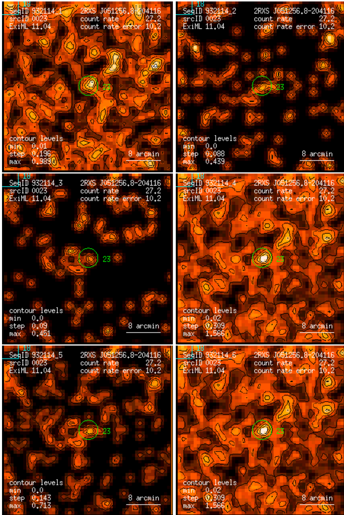
Figure 23: RASS 932114: detection 0023: band rate images, Gaussian filter: (1) PSPC channels 11 – 41, (2) 52 – 90, (3) 91 – 201, (4) 11 – 235, (5) 52 – 201, (6) 11 – 201. Broad band rates in counts/ks. Band rate contour levels in counts/ks/arcmin 2 .
