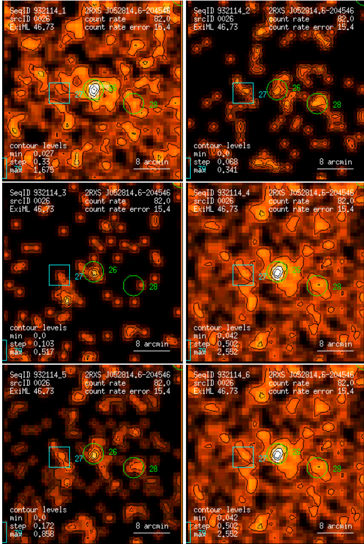
Figure 26: RASS 932114: detection 0026: band rate images, Gaussian filter: (1) PSPC channels 11 – 41, (2) 52 – 90, (3) 91 – 201, (4) 11 – 235, (5) 52 – 201, (6) 11 – 201. Broad band rates in counts/ks. Band rate contour levels in counts/ks/arcmin 2 .
