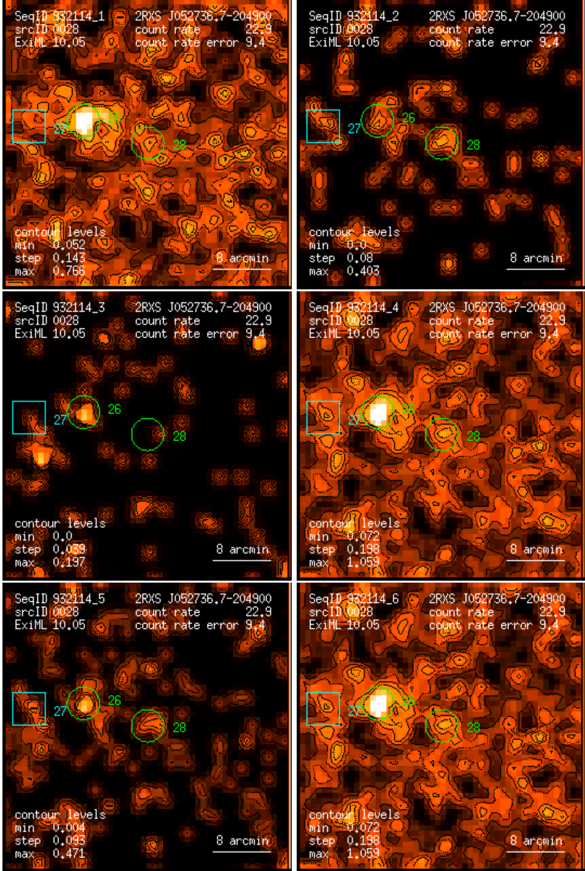
Figure 28: RASS 932114: detection 0028: band rate images, Gaussian filter: (1) PSPC channels 11 – 41, (2) 52 – 90, (3) 91 – 201, (4) 11 – 235, (5) 52 – 201, (6) 11 – 201. Broad band rates in counts/ks. Band rate contour levels in counts/ks/arcmin 2 .
