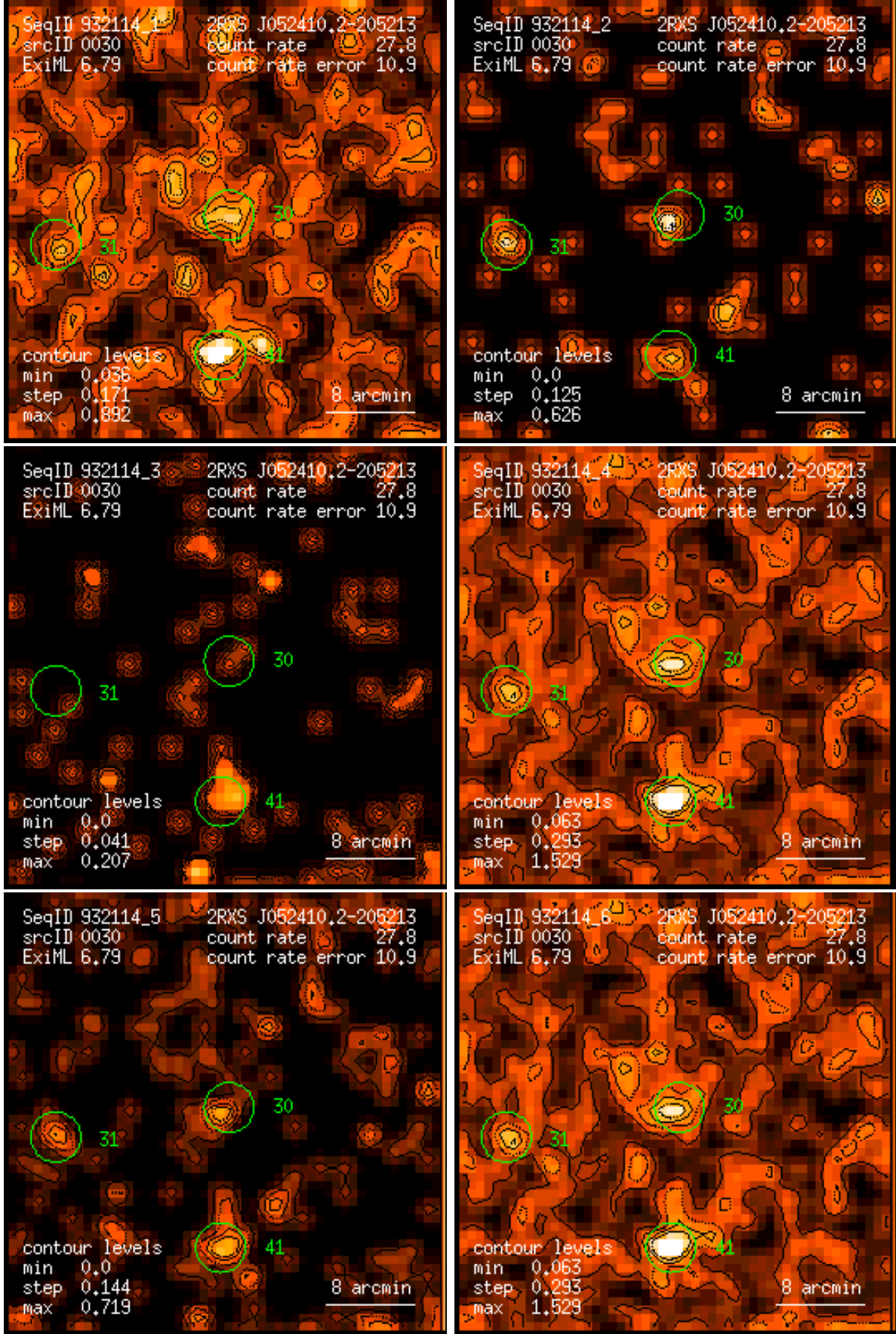
Figure 30: RASS 932114: detection 0030: band rate images, Gaussian filter: (1) PSPC channels 11 – 41, (2) 52 – 90, (3) 91 – 201, (4) 11 – 235, (5) 52 – 201, (6) 11 – 201. Broad band rates in counts/ks. Band rate contour levels in counts/ks/arcmin 2 .
