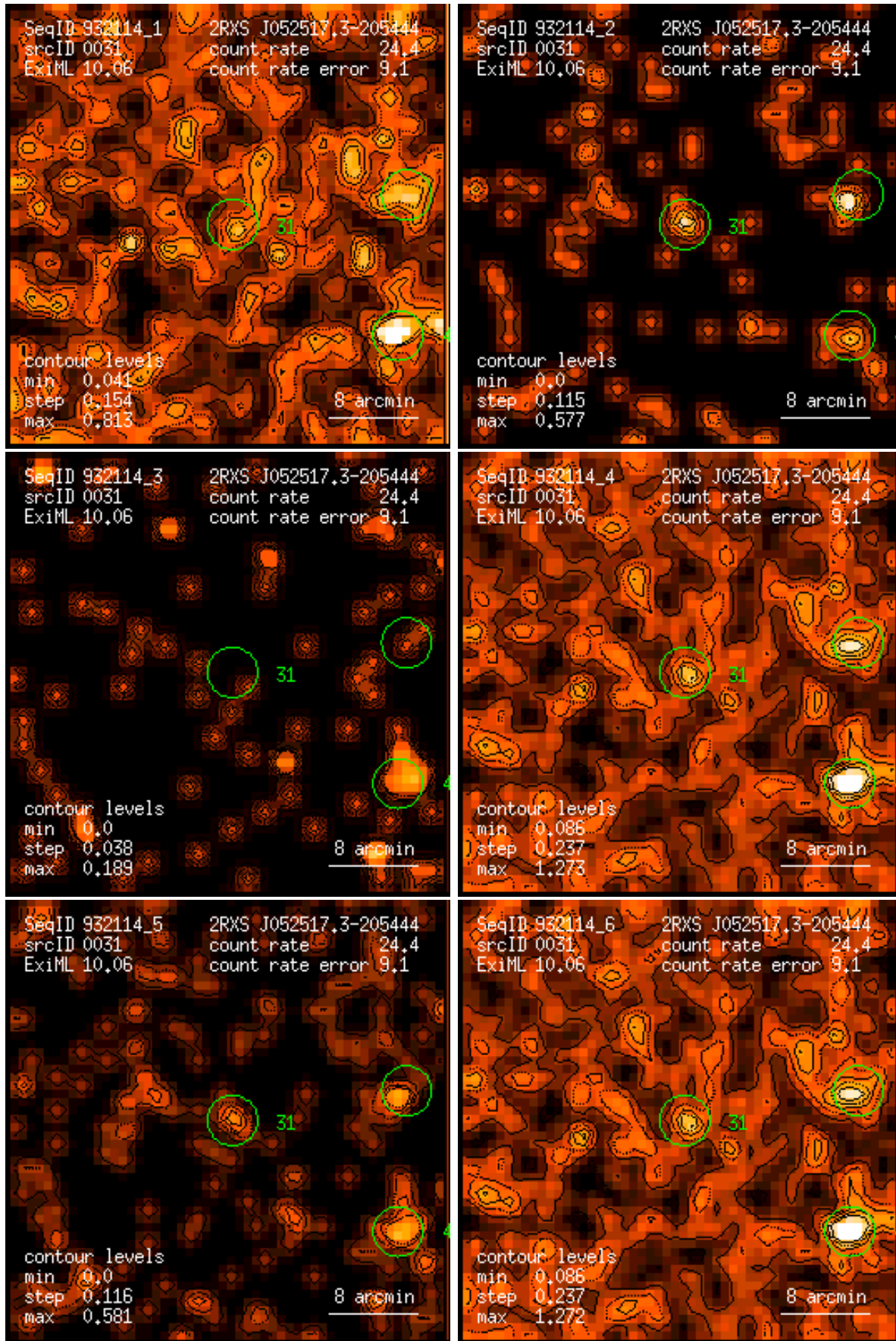
Figure 31: RASS 932114: detection 0031: band rate images, Gaussian filter: (1) PSPC channels 11 – 41, (2) 52 – 90, (3) 91 – 201, (4) 11 – 235, (5) 52 – 201, (6) 11 – 201. Broad band rates in counts/ks. Band rate contour levels in counts/ks/arcmin 2 .
