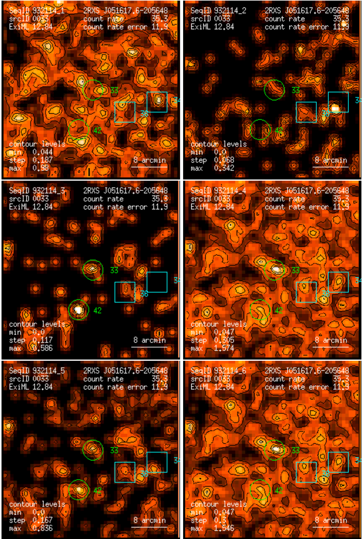
Figure 33: RASS 932114: detection 0033: band rate images, Gaussian filter: (1) PSPC channels 11 – 41, (2) 52 – 90, (3) 91 – 201, (4) 11 – 235, (5) 52 – 201, (6) 11 – 201. Broad band rates in counts/ks. Band rate contour levels in counts/ks/arcmin 2 .
