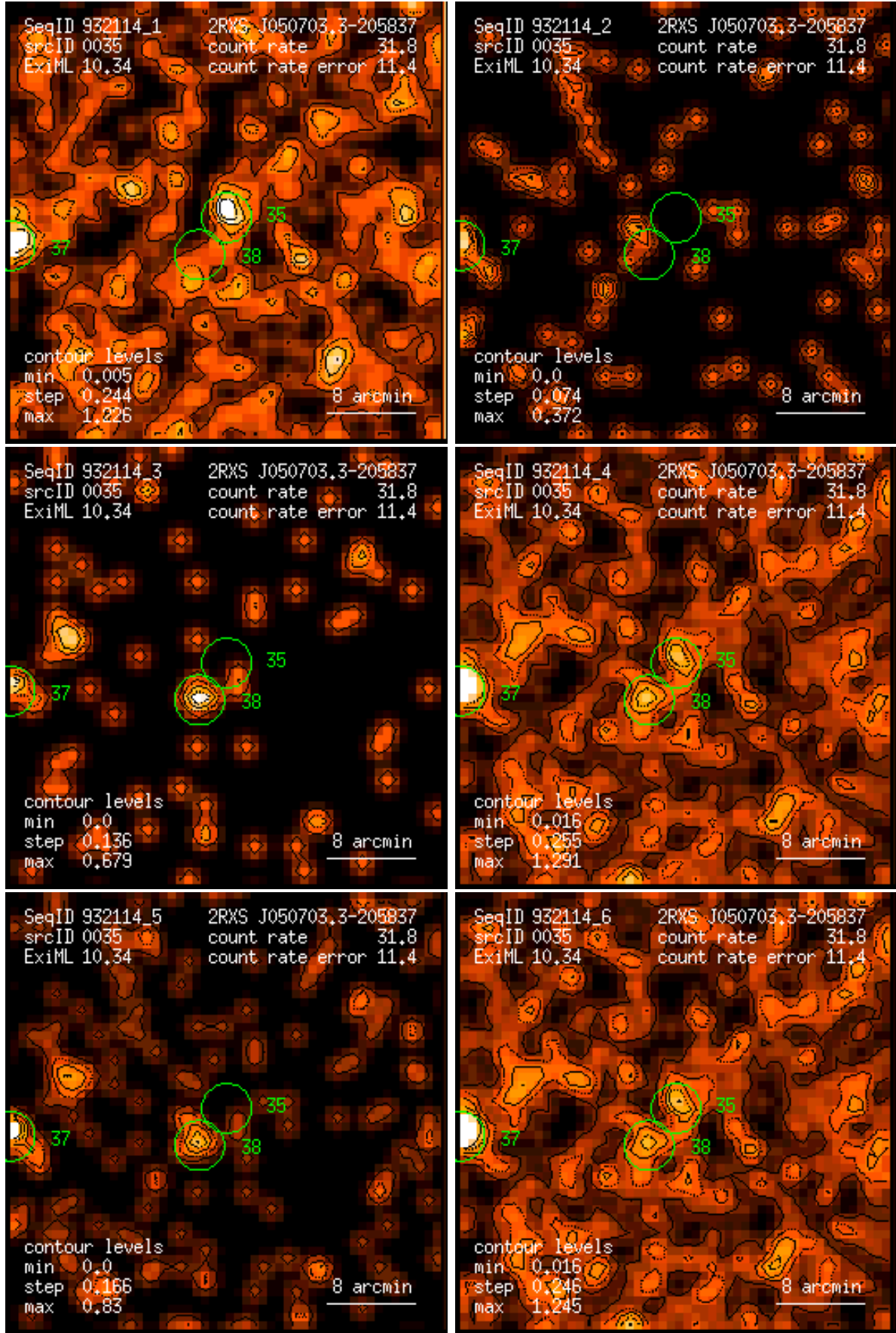
Figure 35: RASS 932114: detection 0035: band rate images, Gaussian filter: (1) PSPC channels 11 – 41, (2) 52 – 90, (3) 91 – 201, (4) 11 – 235, (5) 52 – 201, (6) 11 – 201. Broad band rates in counts/ks. Band rate contour levels in counts/ks/arcmin 2 .
