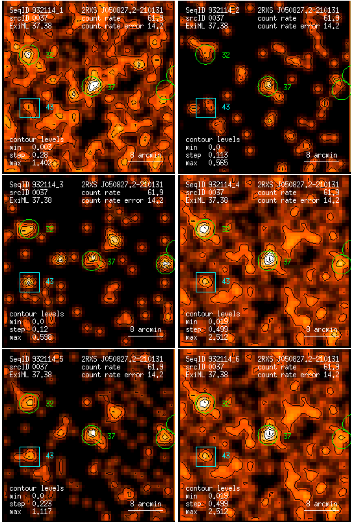
Figure 37: RASS 932114: detection 0037: band rate images, Gaussian filter: (1) PSPC channels 11 – 41, (2) 52 – 90, (3) 91 – 201, (4) 11 – 235, (5) 52 – 201, (6) 11 – 201. Broad band rates in counts/ks. Band rate contour levels in counts/ks/arcmin 2 .
