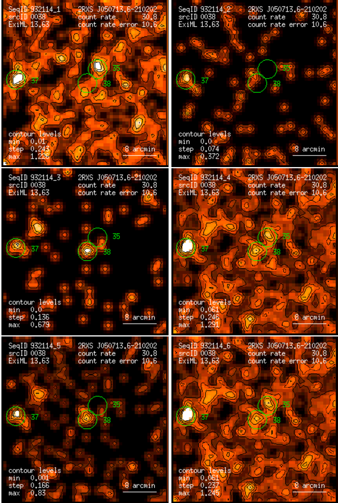
Figure 38: RASS 932114: detection 0038: band rate images, Gaussian filter: (1) PSPC channels 11 – 41, (2) 52 – 90, (3) 91 – 201, (4) 11 – 235, (5) 52 – 201, (6) 11 – 201. Broad band rates in counts/ks. Band rate contour levels in counts/ks/arcmin 2 .
