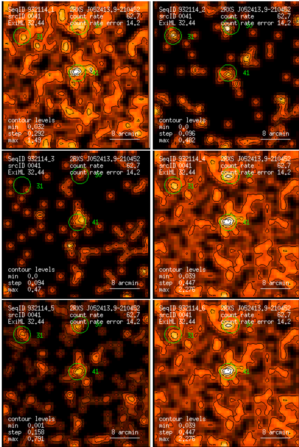
Figure 41: RASS 932114: detection 0041: band rate images, Gaussian filter: (1) PSPC channels 11 – 41, (2) 52 – 90, (3) 91 – 201, (4) 11 – 235, (5) 52 – 201, (6) 11 – 201. Broad band rates in counts/ks. Band rate contour levels in counts/ks/arcmin 2 .
