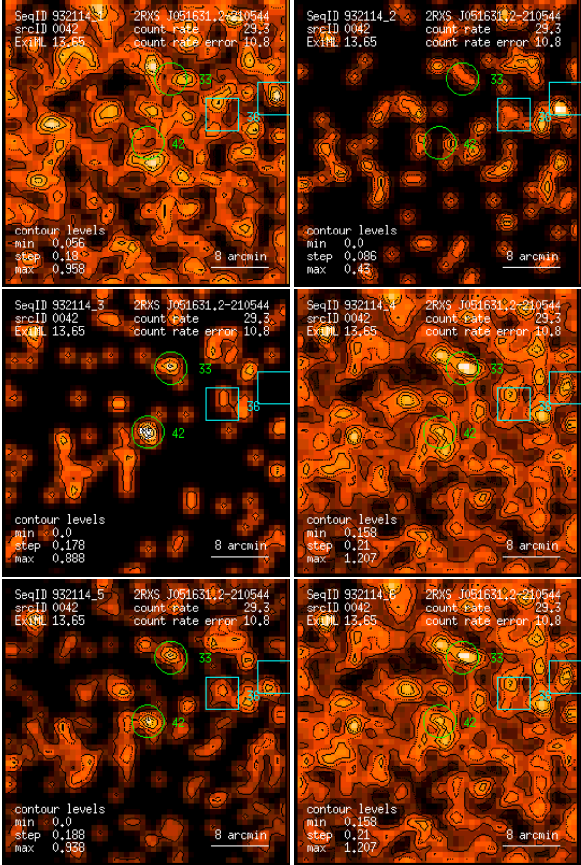
Figure 42: RASS 932114: detection 0042: band rate images, Gaussian filter: (1) PSPC channels 11 – 41, (2) 52 – 90, (3) 91 – 201, (4) 11 – 235, (5) 52 – 201, (6) 11 – 201. Broad band rates in counts/ks. Band rate contour levels in counts/ks/arcmin 2 .
