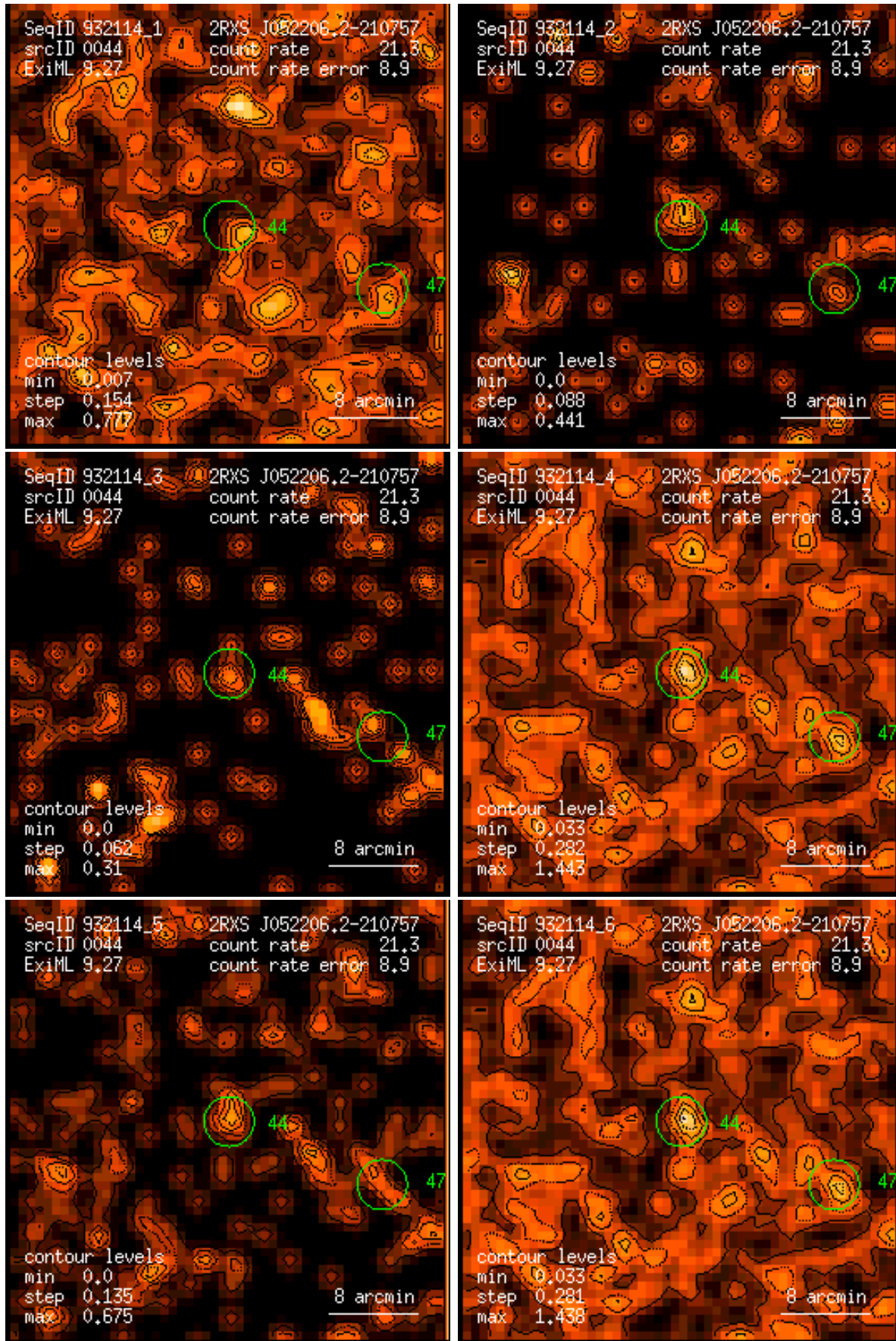
Figure 44: RASS 932114: detection 0044: band rate images, Gaussian filter: (1) PSPC channels 11 – 41, (2) 52 – 90, (3) 91 – 201, (4) 11 – 235, (5) 52 – 201, (6) 11 – 201. Broad band rates in counts/ks. Band rate contour levels in counts/ks/arcmin 2 .
