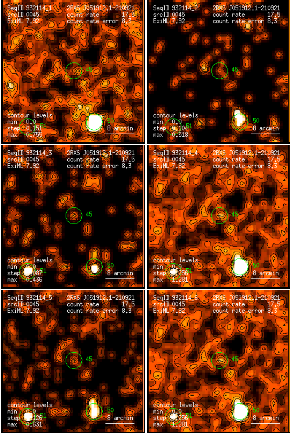
Figure 45: RASS 932114: detection 0045: band rate images, Gaussian filter: (1) PSPC channels 11 – 41, (2) 52 – 90, (3) 91 – 201, (4) 11 – 235, (5) 52 – 201, (6) 11 – 201. Broad band rates in counts/ks. Band rate contour levels in counts/ks/arcmin 2 .
