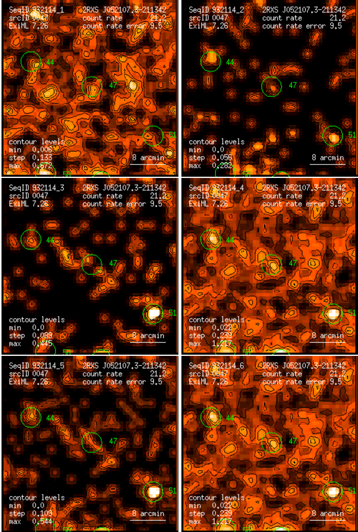
Figure 47: RASS 932114: detection 0047: band rate images, Gaussian filter: (1) PSPC channels 11 – 41, (2) 52 – 90, (3) 91 – 201, (4) 11 – 235, (5) 52 – 201, (6) 11 – 201. Broad band rates in counts/ks. Band rate contour levels in counts/ks/arcmin 2 .
