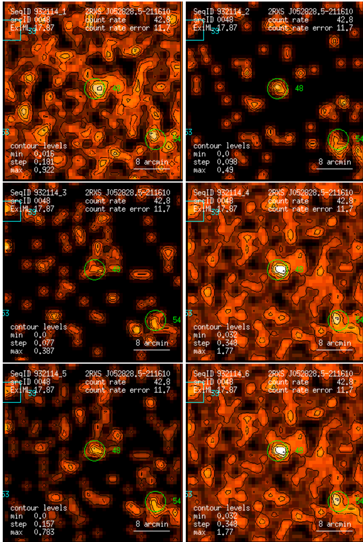
Figure 48: RASS 932114: detection 0048: band rate images, Gaussian filter: (1) PSPC channels 11 – 41, (2) 52 – 90, (3) 91 – 201, (4) 11 – 235, (5) 52 – 201, (6) 11 – 201. Broad band rates in counts/ks. Band rate contour levels in counts/ks/arcmin 2 .
