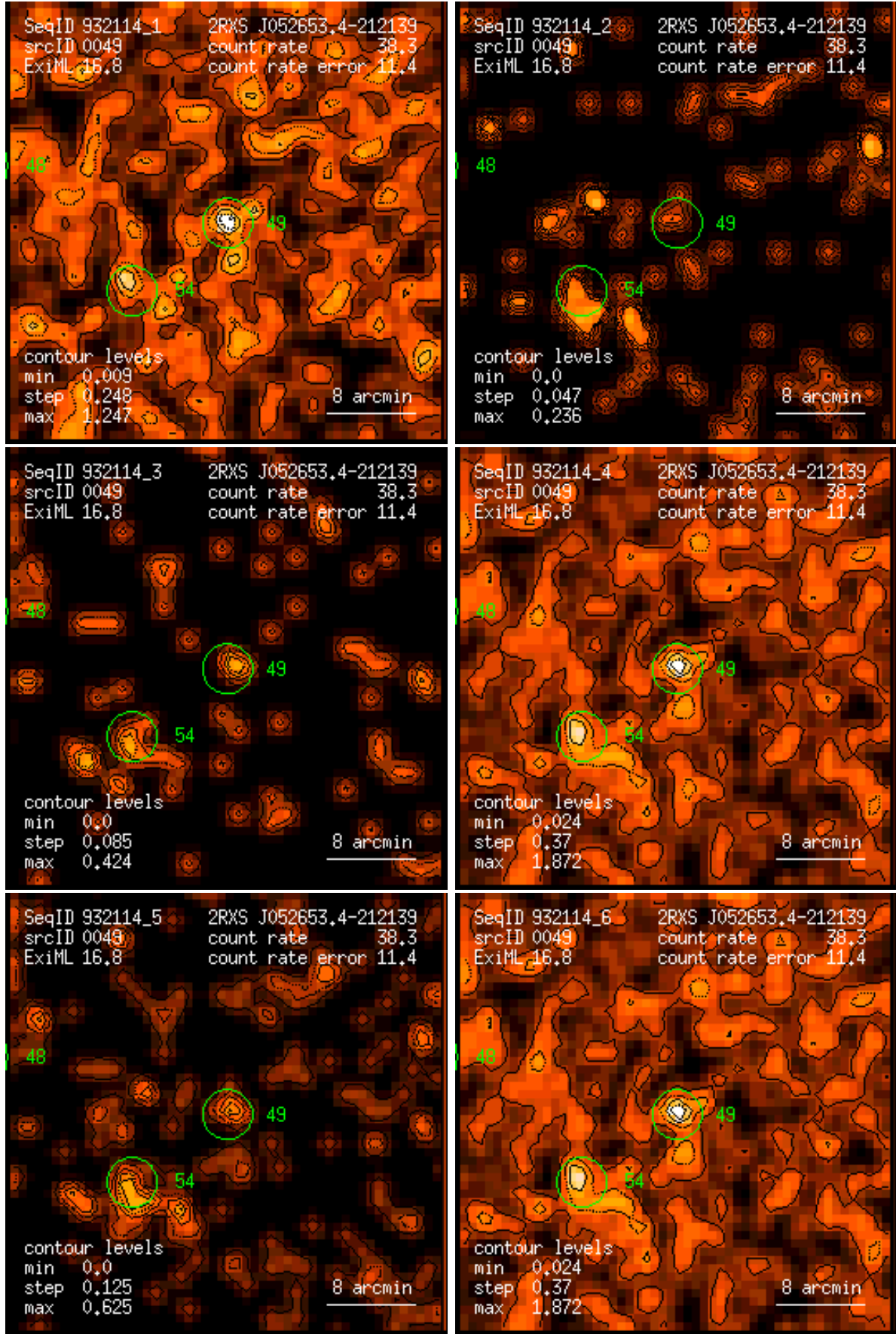
Figure 49: RASS 932114: detection 0049: band rate images, Gaussian filter: (1) PSPC channels 11 – 41, (2) 52 – 90, (3) 91 – 201, (4) 11 – 235, (5) 52 – 201, (6) 11 – 201. Broad band rates in counts/ks. Band rate contour levels in counts/ks/arcmin 2 .
