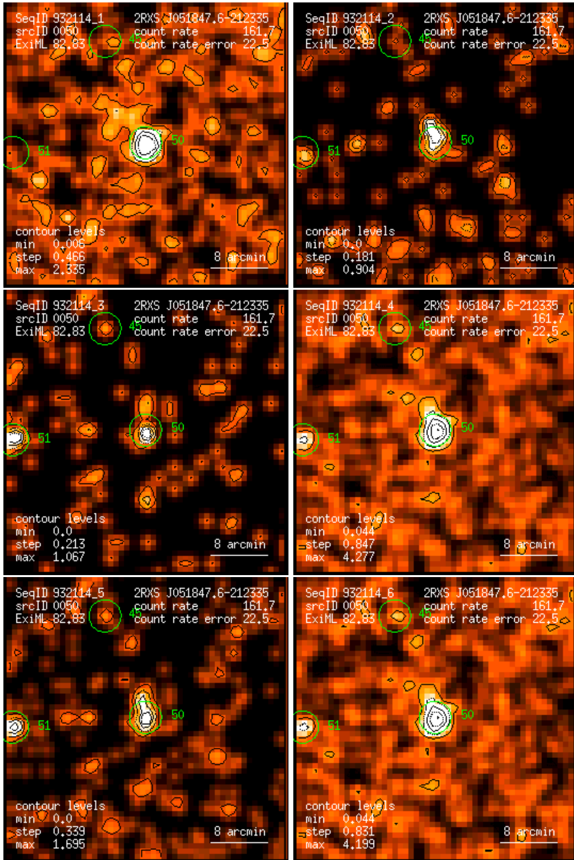
Figure 50: RASS 932114: detection 0050: band rate images, Gaussian filter: (1) PSPC channels 11 – 41, (2) 52 – 90, (3) 91 – 201, (4) 11 – 235, (5) 52 – 201, (6) 11 – 201. Broad band rates in counts/ks. Band rate contour levels in counts/ks/arcmin 2 .
