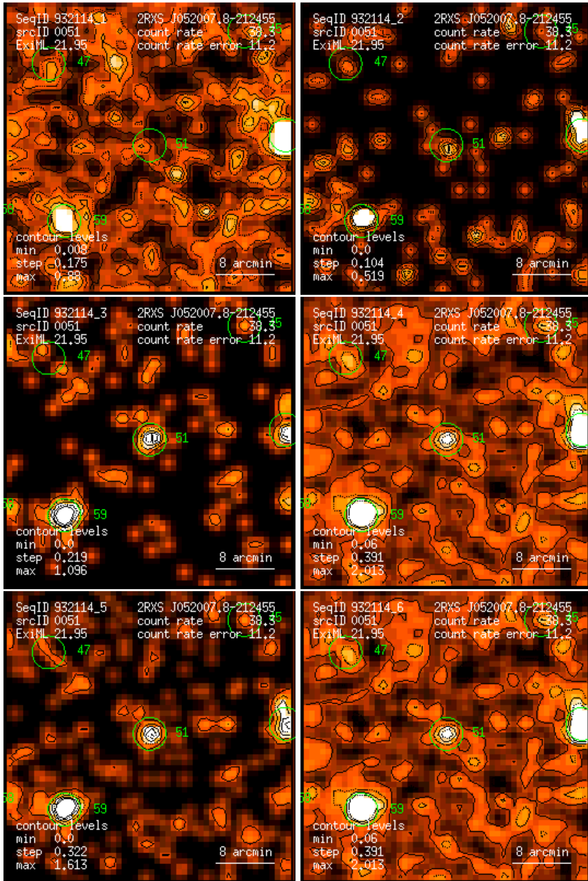
Figure 51: RASS 932114: detection 0051: band rate images, Gaussian filter: (1) PSPC channels 11 – 41, (2) 52 – 90, (3) 91 – 201, (4) 11 – 235, (5) 52 – 201, (6) 11 – 201. Broad band rates in counts/ks. Band rate contour levels in counts/ks/arcmin 2 .
