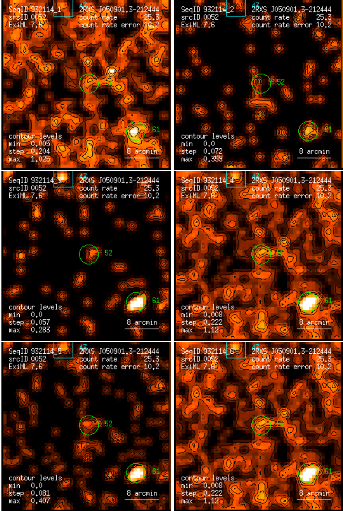
Figure 52: RASS 932114: detection 0052: band rate images, Gaussian filter: (1) PSPC channels 11 – 41, (2) 52 – 90, (3) 91 – 201, (4) 11 – 235, (5) 52 – 201, (6) 11 – 201. Broad band rates in counts/ks. Band rate contour levels in counts/ks/arcmin 2 .
