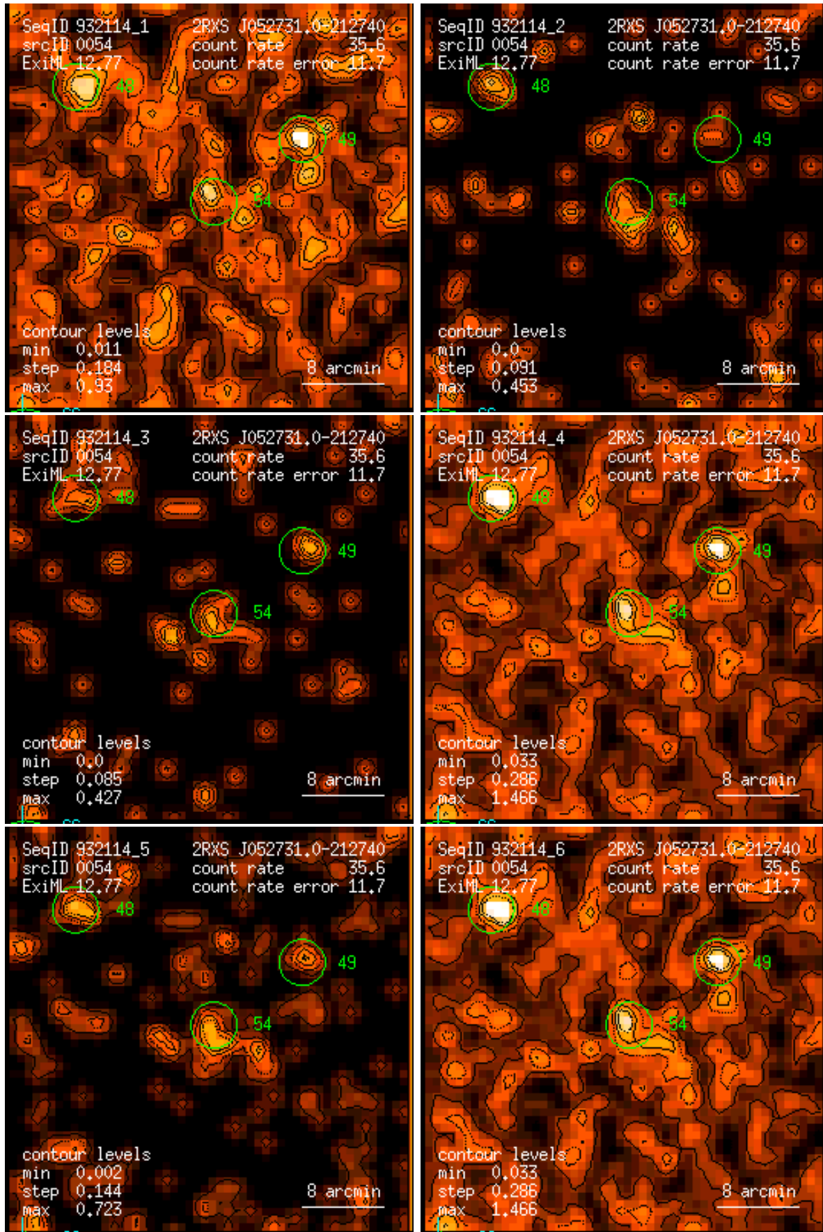
Figure 54: RASS 932114: detection 0054: band rate images, Gaussian filter: (1) PSPC channels 11 – 41, (2) 52 – 90, (3) 91 – 201, (4) 11 – 235, (5) 52 – 201, (6) 11 – 201. Broad band rates in counts/ks. Band rate contour levels in counts/ks/arcmin 2 .
