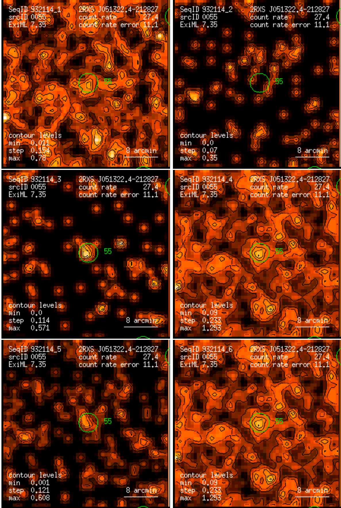
Figure 55: RASS 932114: detection 0055: band rate images, Gaussian filter: (1) PSPC channels 11 – 41, (2) 52 – 90, (3) 91 – 201, (4) 11 – 235, (5) 52 – 201, (6) 11 – 201. Broad band rates in counts/ks. Band rate contour levels in counts/ks/arcmin 2 .
