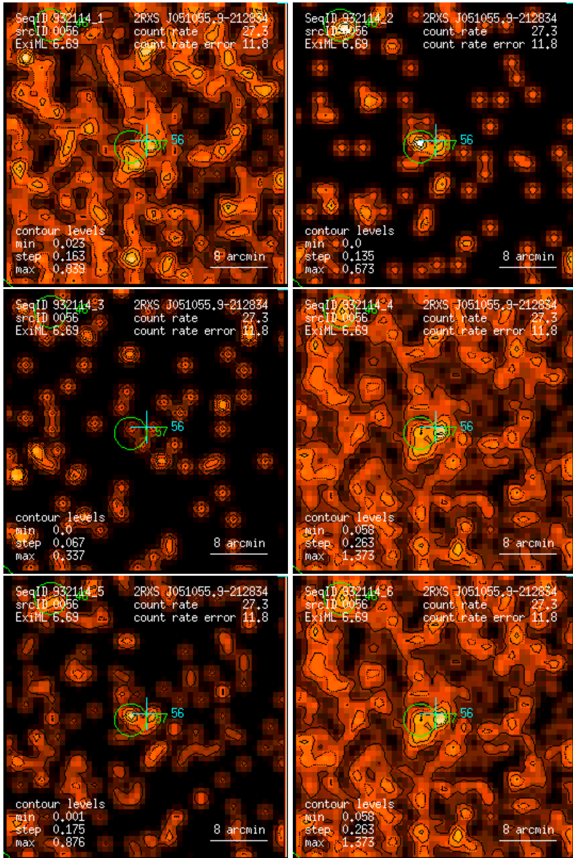
Figure 56: RASS 932114: detection 0056: band rate images, Gaussian filter: (1) PSPC channels 11 – 41, (2) 52 – 90, (3) 91 – 201, (4) 11 – 235, (5) 52 – 201, (6) 11 – 201. Broad band rates in counts/ks. Band rate contour levels in counts/ks/arcmin 2 .
