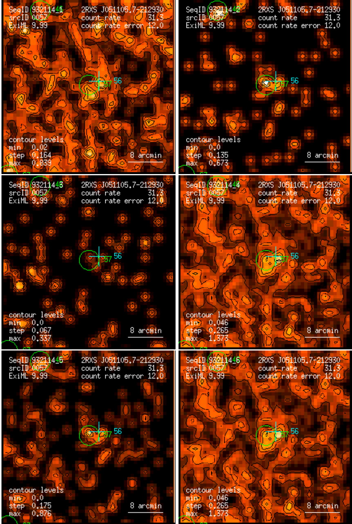
Figure 57: RASS 932114: detection 0057: band rate images, Gaussian filter: (1) PSPC channels 11 – 41, (2) 52 – 90, (3) 91 – 201, (4) 11 – 235, (5) 52 – 201, (6) 11 – 201. Broad band rates in counts/ks. Band rate contour levels in counts/ks/arcmin 2 .
